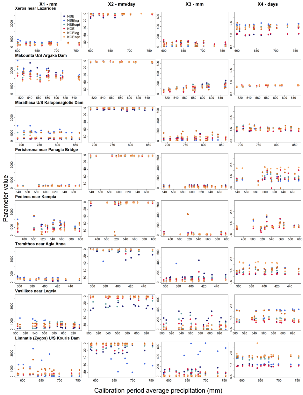
670 Figure A1: Values of the four parameters of the GR4J model optimized with six objective functions for the 14 five-year calibration periods for eight watersheds. The mean precipitation of each five-year calibration period is shown on the horizontal axis.
