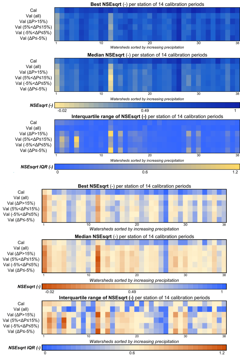
Figure 3 Heatmap with the best (top), median (middle) and interquartile range (IQR) (bottom) of NSEsqr (-) for each watershed, sorted by increasing long-term annual average precipitation (columns) and each calibration-validation set of runs (rows). The values of NSEsqr or the IQR for each cell in the heatmap are computed as averages of the values from the 14 5-year calibration runs, the 13 validation runs for each of the 14 calibration runs. i.e., Val (all), and the validation runs corresponding to each of the four precipitation change classes, as specified in Table 1.
