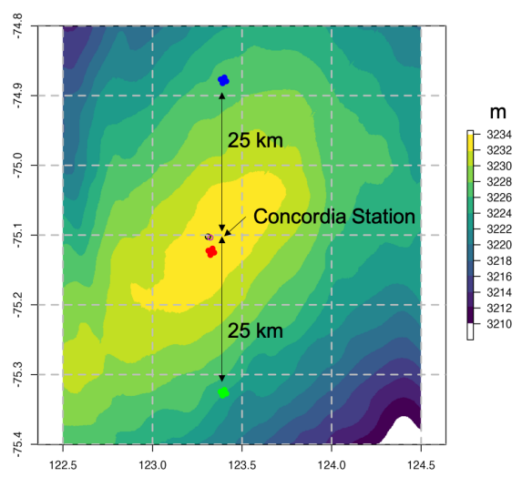
220 Figure 2. Elevation of the Dome C area (colours from REMA, Howat et al., 2022) and locations of the northern (FRA-N, blue circles) and southern (FRA-S, green circles) French stake farms. The purple, black (very close to each other), and red circles are the stake farms near Concordia Station shown in Fig. 1. Longitude and latitude are shown in decimal degrees.
