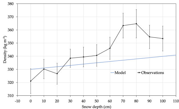
270 Figure 3. Observed snow density from 0 to 1 m depth at 10 cm intervals (black line) near Concordia Station for the 2014-2023 period, and 95% confidence intervals (bars); the model (blue line) is the Eq. 1.
