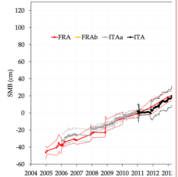
Deleted: Figure 4. Cumulative SMB from the Italian and French stake farms near Concordia Station with respect to the beginning of 2011. Continuous coloured lines connect the mean values while the dashed lines indicate \pm 1 standard deviation of each dataset.
