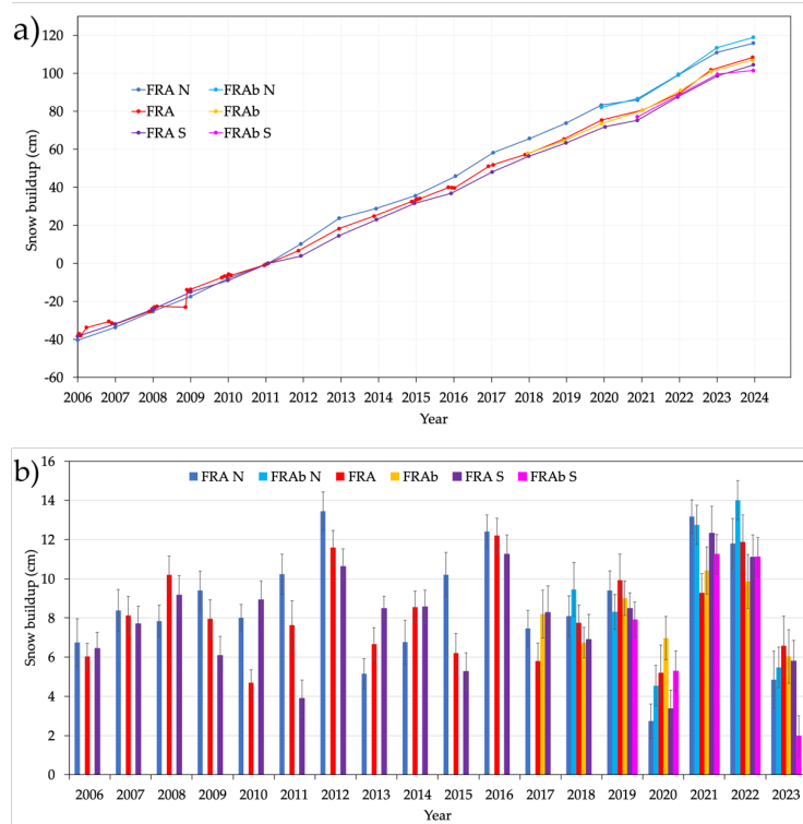
515 Figure 6. (a) Cumulative snow buildup from the French stake farms near Concordia Station, and in the southern and northern sites for the 2006-2023 period, with respect to 2011; (b) yearly snow buildup derived from (a), the uncertainty bars indicate the standard errors of the mean values.
