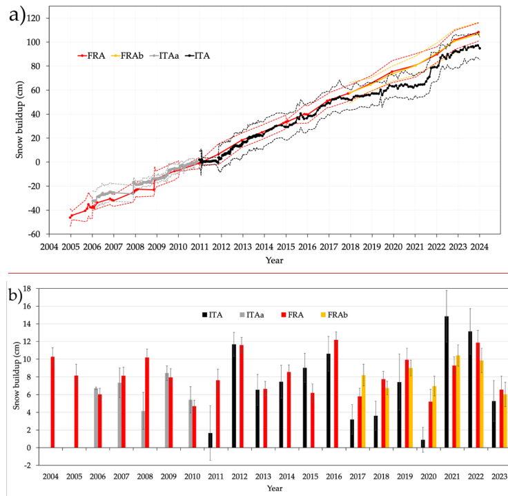
Figure 4. (a) Cumulative snow buildup from the Italian and French stake farms near Concordia Station with respect to the beginning of 2011. Continuous coloured lines connect the mean values while the dashed lines indicate \pm 1 standard deviation of each dataset; (b) yearly mean snow buildup from the Italian and French stake farms near Concordia Station. The uncertainty bars indicate the standard errors of the mean values.
