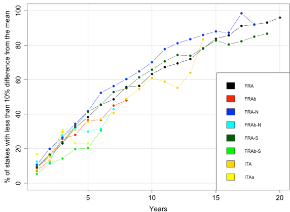
Figure 2. Number of stakes (in %) with less than 10% difference in accumulation from the mean of the stake farm for different year intervals.
