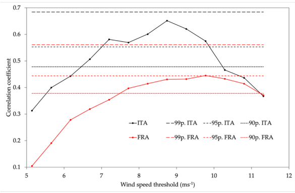
Figure 10. Linear correlation coefficients between the yearly fraction of stakes with negative and zero SB and the frequency of wind speed values at the AWS above certain thresholds. 99%, 95%, and 90% confidence levels for each stake farm are shown.
