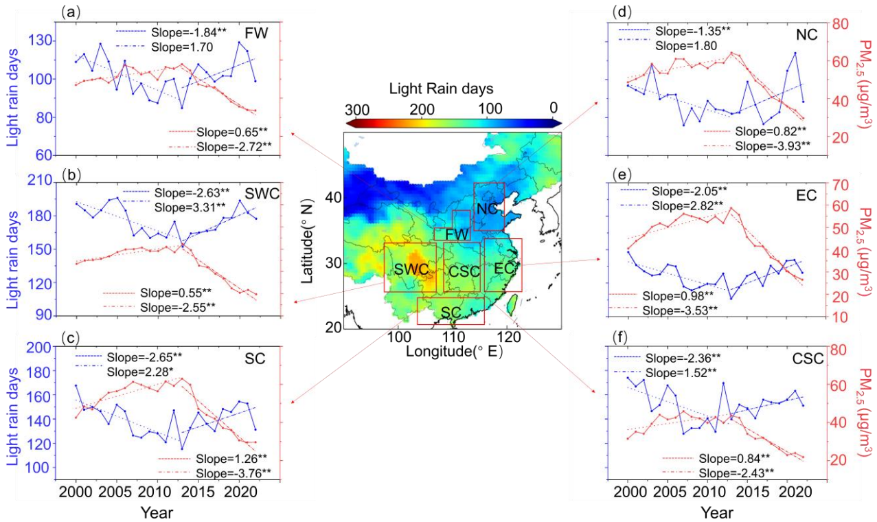
Figure 2. The fitted variation trends of light rain days (blue lines) and the fitted variation trends of PM_{2.5} (red lines) in different six selected regions. The middle map shows the spatial distribution of average light rain days during 2000–2022 and the six selected study regions.
