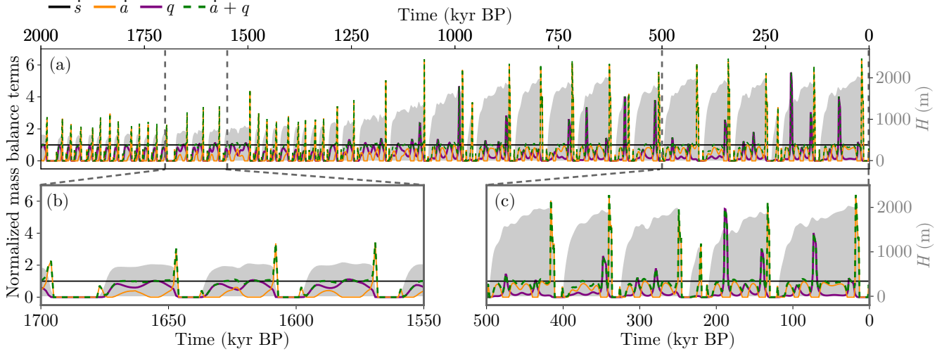
Figure 5. Results from BASE experiment showing the evolution of the ice thickness H (in gray) and mass balance terms (snowfall \dot{s} , ablation \dot{a} and ice discharge q normalized by \dot{s} , as defined in Appendix A3) for different ranges of time.
