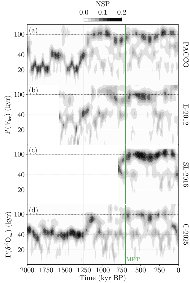
Figure 7. NSP of ice volume V_{ice} and sea-water component (\delta^{18}O_{sw}) of \delta^{18}O at each period ( P ) as a function of time from (a) BASE experiment, (b) Elderfield et al. (2012, E-2012), (c) Spratt and Lisiecki (2016, SL-2016) and (d) Clark et al. (2025, C-2025). Vertical green lines correspond to the interval associated with the occurrence of the MPT (Clark et al., 2006).
