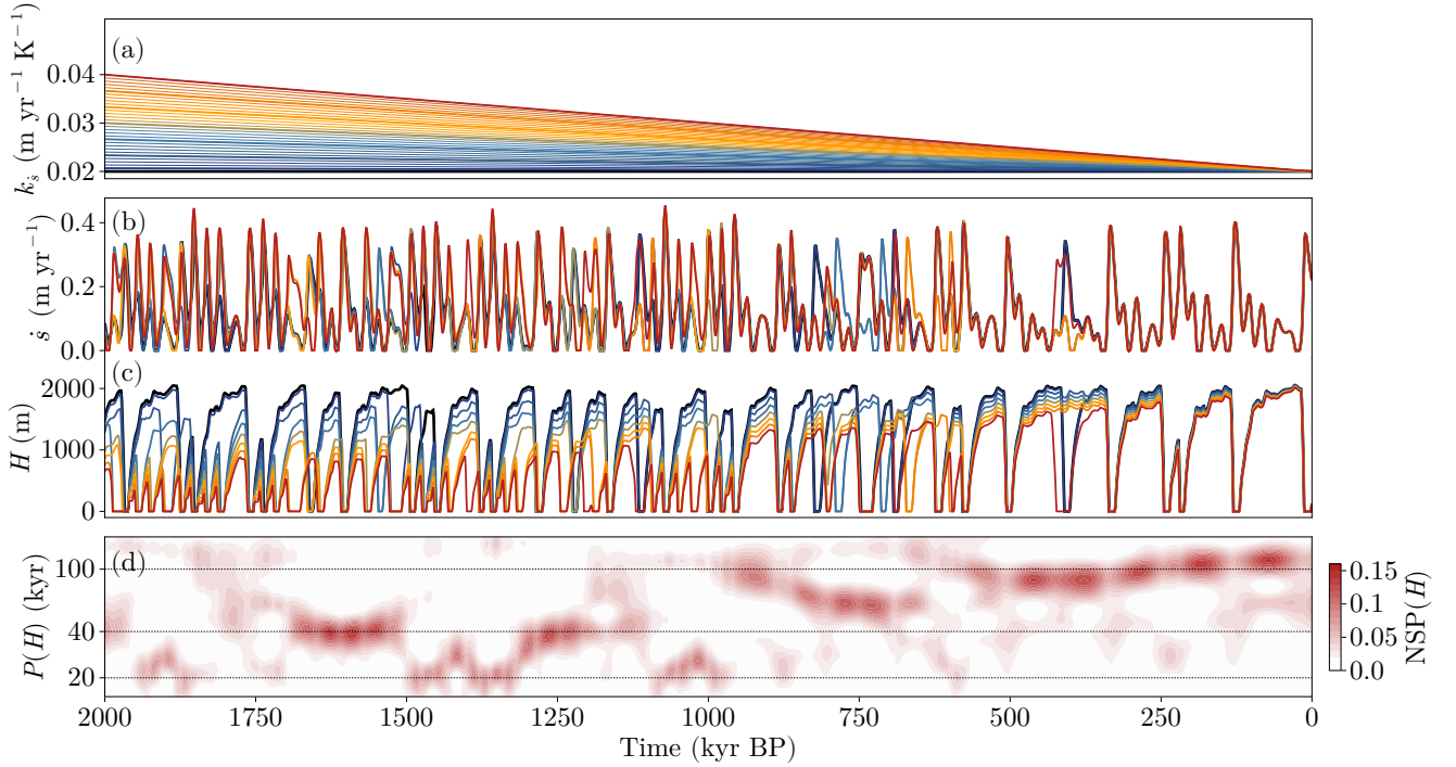
Figure 15. Time series of (colors) TREND-S experiment and (black) NOSEDIM-low experiment. (a) sensitivity of accumulation to temper- ature k_s , (b) snowfall \dot{s} , (c) ice thickness H and (d) wavelet transform of H for the maximum decreasing trend (red) case. Note that in (b) and (c) only the curves highlighted in (a) are plotted.
