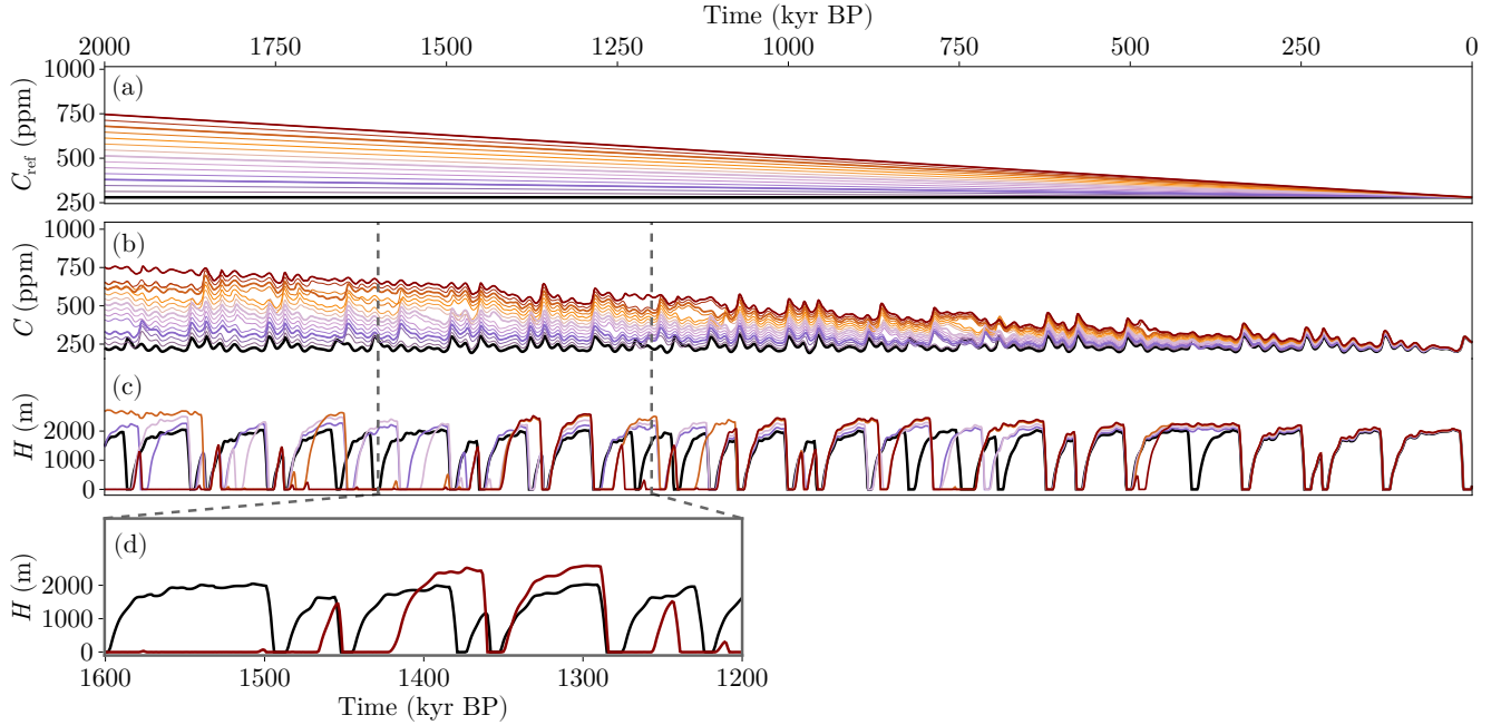
Figure 14. Time series of (colors) TREND-C experiment and (black) NOSEDIM-low experiment. (a) reference carbon dioxide C_{\text{ref}} , (b) carbon dioxide C , (c) ice thickness H and (d) zoom of the range squared in (c) for the two extreme cases. Note that in (c) only the curves highlighted in (a) and (b) are plotted.
