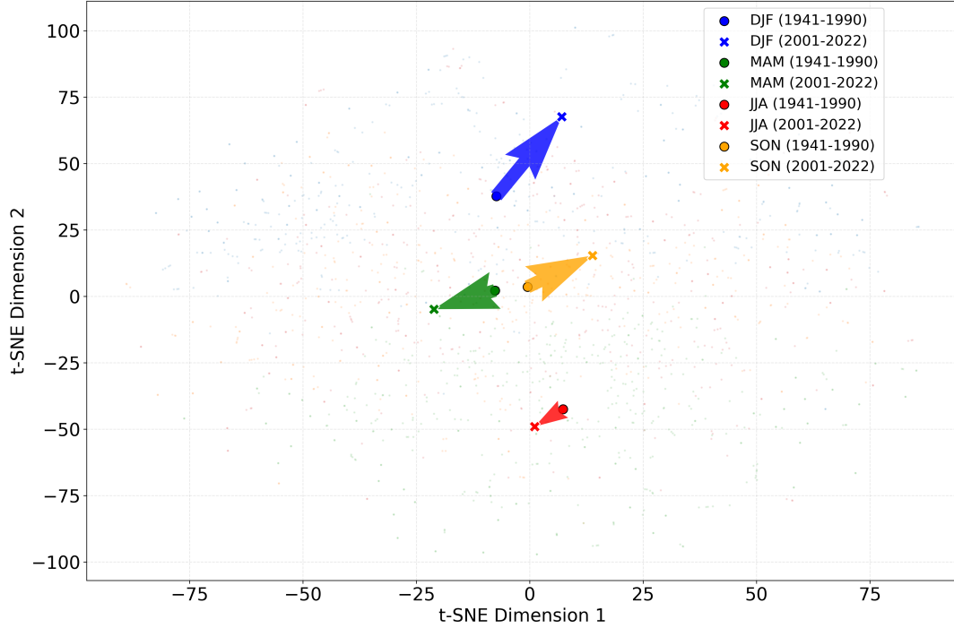
Figure A8. [.. 116 ] Temporal evolution of seasonal atmospheric patterns in the VAE latent space [.. 117 ] using detrended data . [.. 118 ] [.. 119 ] Vectors indicate the shift in mean latent embeddings for heatwave [.. 119 ] samples between 1941–1990 and 2001–2022 for Winter (blue), Spring (green), Summer (red), and Autumn (orange). [.. 120 ] All shifts are statistically significant ( p < 0.001 ). Winter patterns exhibit the [.. 121 ] most substantial displacement (Mahalanobis distance D = 1.40 ), indicating that changes in this dataset reflect primarily dynamical reorganizations.
