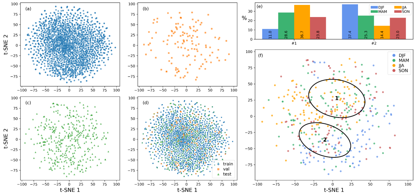
Figure A1. [.. 106 ] t-SNE representation of the latent [.. 107 ] space with random-split data ( [.. 108 ] 0.8/0.05/0.15) [.. 109 ] . Following our workflow ( [.. 110 ] testing with more than 2 components) [.. 111 ] , a 2-component GMM provided the [.. 112 ] best fit, as it was closest to a [.. 113 ] single Gaussian distribution and [.. 114 ] thus better captured the smooth latent-space structure. [.. 115 ] While this approach provides a smoother latent space, summer heatwaves still accumulate more closely together. This confirms that the clustering is not simply an artifact in the time series but reflects consistent structural patterns across periods.
