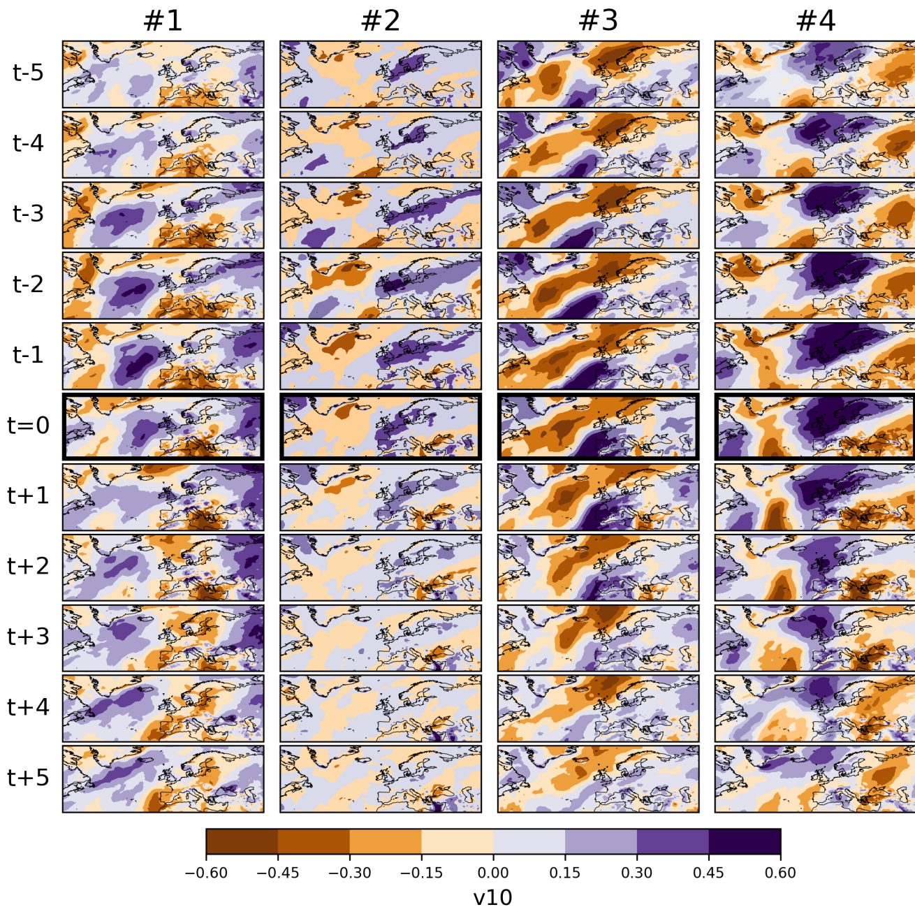
Figure 14. Same as Figure 7, but for standardized 10-meter [.87] northward wind component ( v10 ) anomaly.
