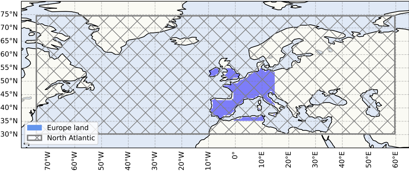
Geographical domains used to identify heatwave onset dates and train the VAE model. The shaded blue area represents the Western Europe land grid cells used to identify heatwave onset dates based on hot grid points derived from ERA5 temperature fields. These onset dates are then used to extract 11-day heatwave samples, centered on the onset dates, from the broader North Atlantic region (indicated by the hatched gray box), covering the nine variables (multivariate) listed in Table 1. These multivariate heatwave samples are used for training and analysis.
