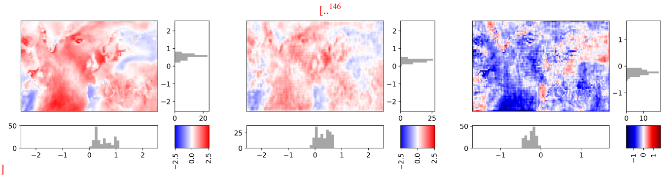
Figure A15. 2-meter temperature for a random sample (left), its VAE reconstruction (middle), and the resulting reconstruction bias (right), each averaged over the time dimension. The histograms below each panel show the distributions of longitudinal and latitudinal values, respectively.
