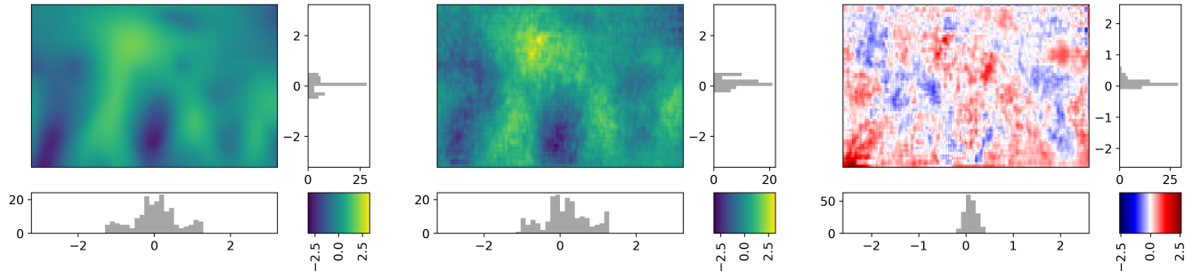
Figure A14. [.. 144 ] Geopotential height at 500 hPa for a random sample (left), its VAE reconstruction (middle), and the resulting reconstruction bias (right), each shown at the onset date. The histograms below [.. 145 ] each panel show the distributions of longitudinal and latitudinal values, respectively.
