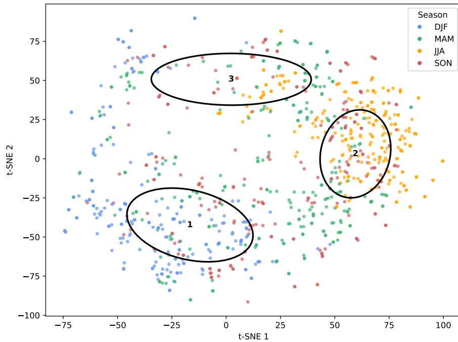
Figure A11. [.. 124 ] t-SNE representation of the latent space with three corresponding GMM components. Each point represents a [.. 125 ] heatwave sample [.. 126 ] . [.. 127 ] Colors represent the [.. 128 ] seasons in which the [.. 129 ] sample onset dates are located.
