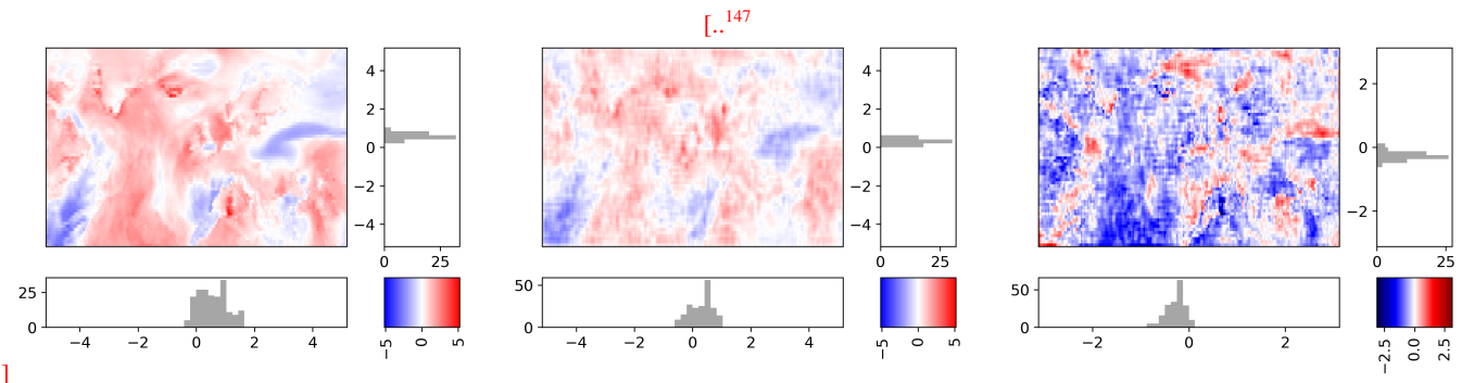
Figure A16. 2-meter temperature for a random sample (left), its VAE reconstruction (middle), and the resulting reconstruction bias (right), each shown at the onset date. The histograms below each panel show the distributions of longitudinal and latitudinal values, respectively.
