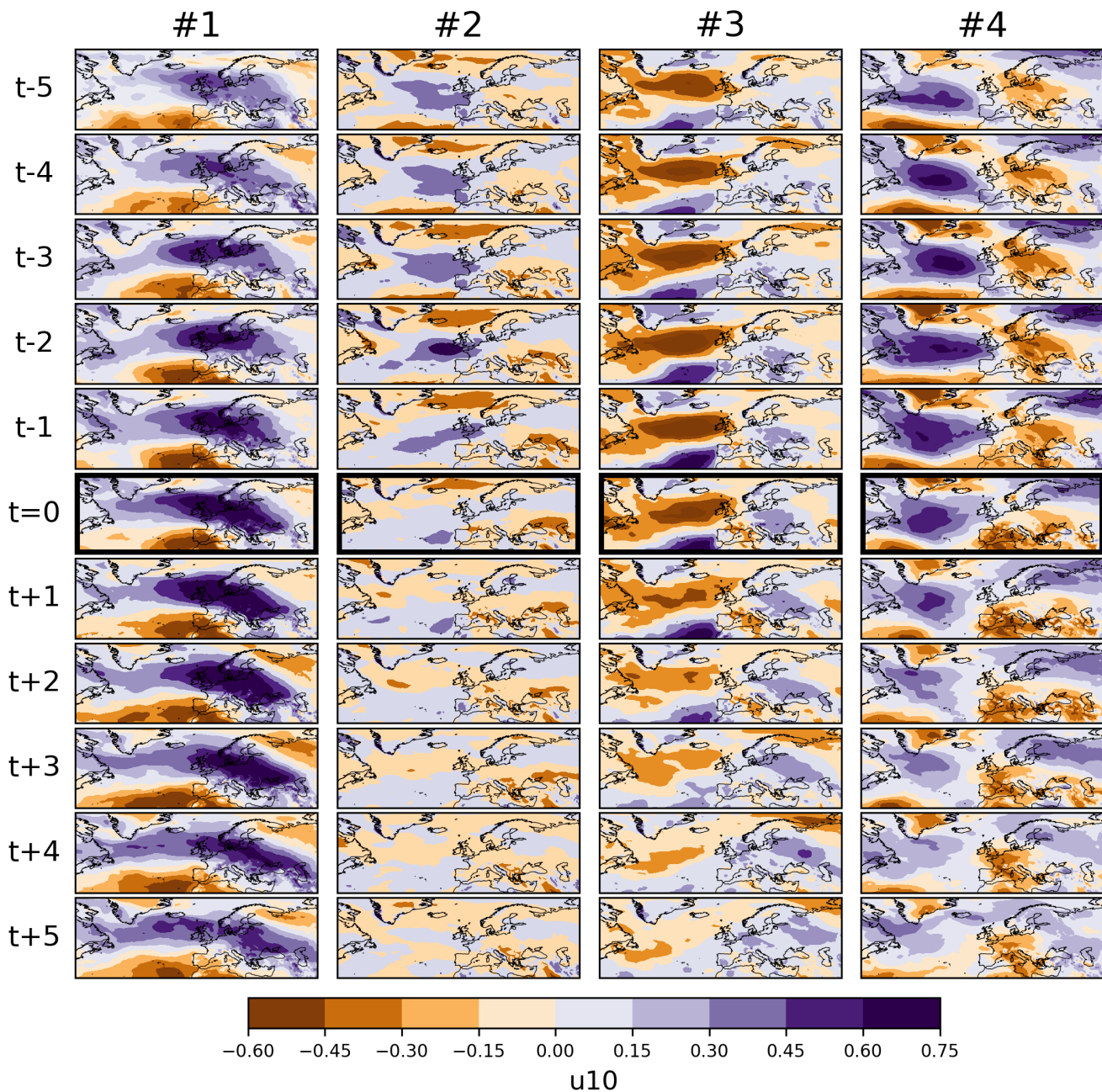
Figure 13. Same as Figure 7, but for standardized 10-meter [.86] eastward wind component ( u10 ) anomaly.
