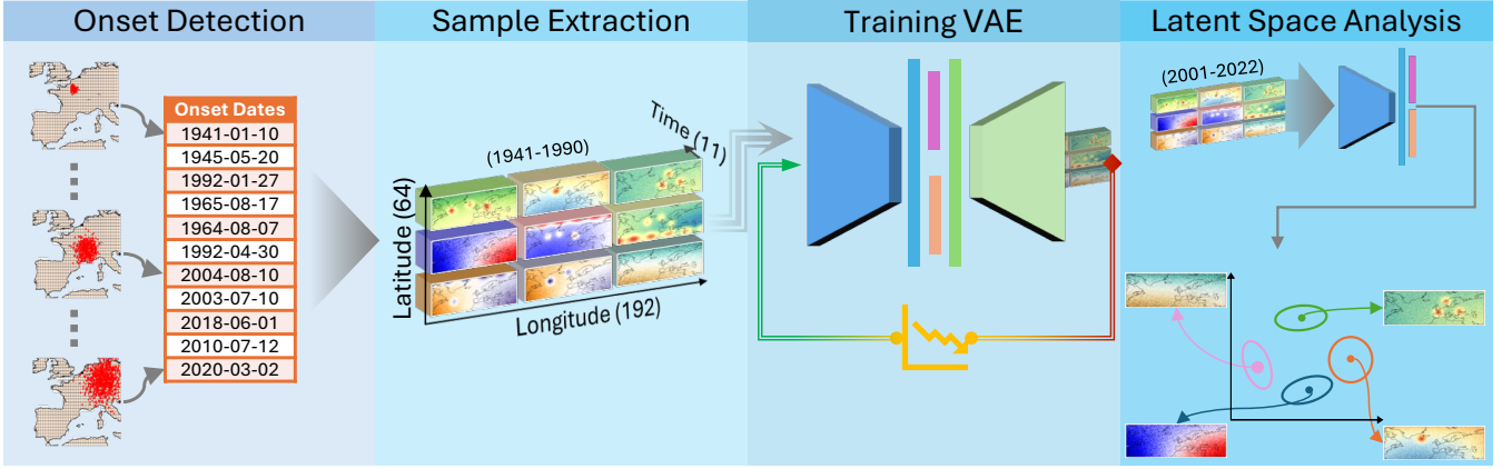
Figure 1. Workflow illustration of the heatwave onset detection and sample extraction process. Detected onset dates over Western Europe are used to extract [.. 53 ] 11-day multivariate heatwave samples from the North Atlantic region, centered on the onset of each event[.. 54 ] . Samples from 1941–1990 are used to train a Variational Autoencoder (VAE) that learns compact representations of the spatiotemporal structure of heatwaves. Subsequently, samples from 2001 [.. 55 ] to 2022 are encoded into the latent space to analyze the evolution and dynamics of recent heatwave events.
