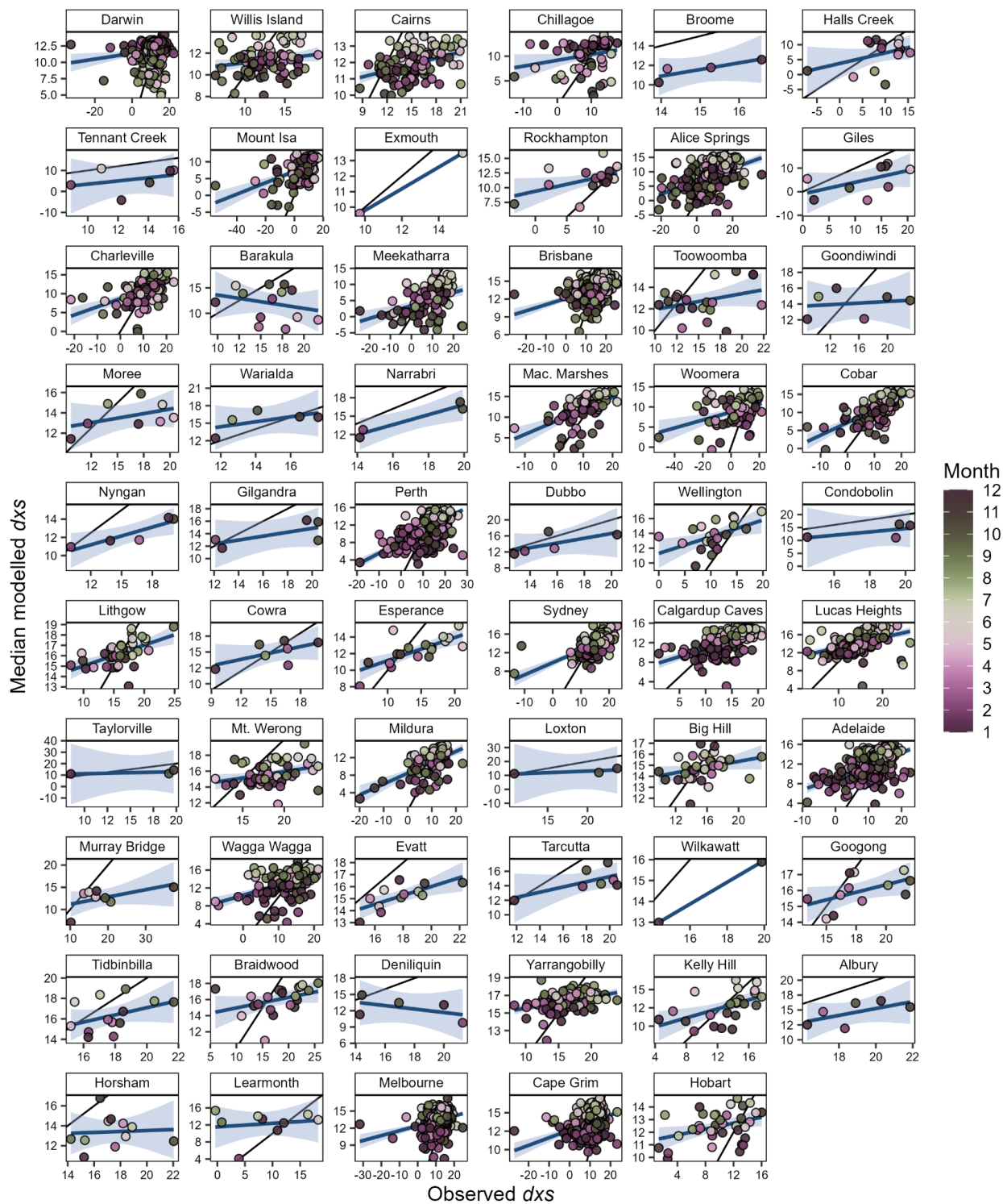
Figure S9: As per Fig. 4 but comparing modelled and observed monthly dxs_P values.
