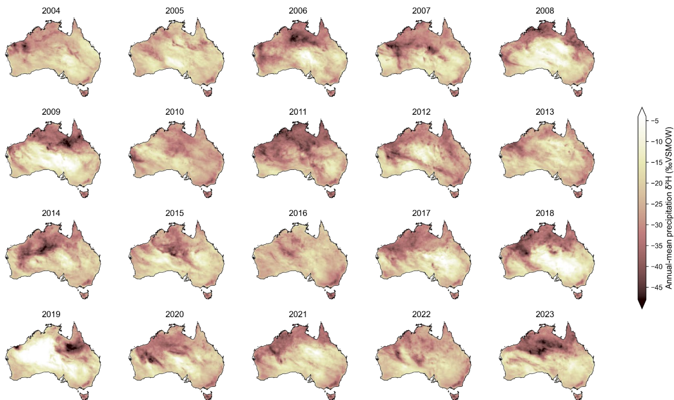
Figure S14: As per Fig. 9 but showing precipitation amount-weighted annual mean \delta^2\text{H}_\text{P} values.
