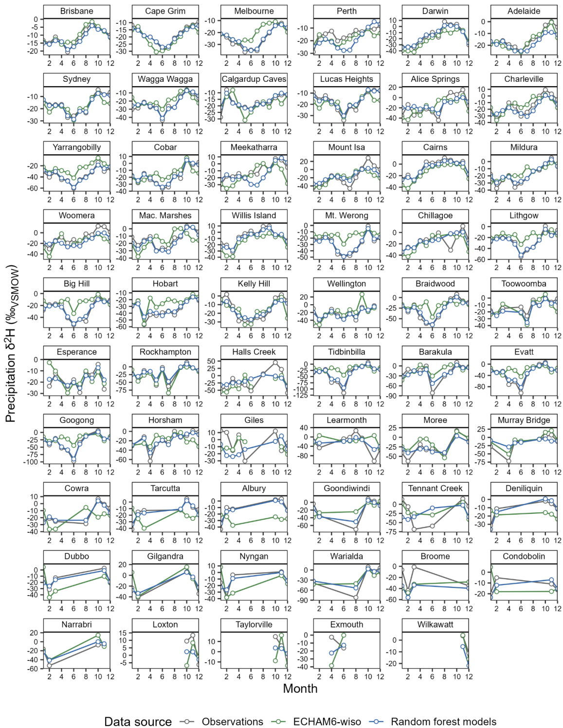
Figure S10: As per Fig. 5 but for the seasonal cycle of \delta^2\text{H}_p .
