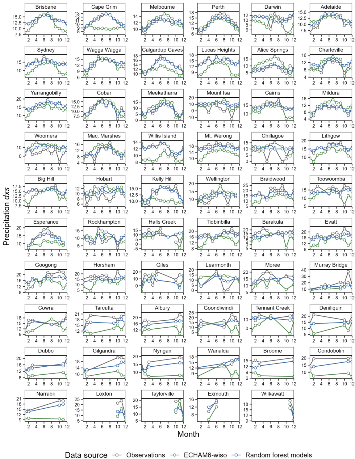
170 Figure S11: As per Fig. 5 but for the seasonal cycle of dx_{SP} .
