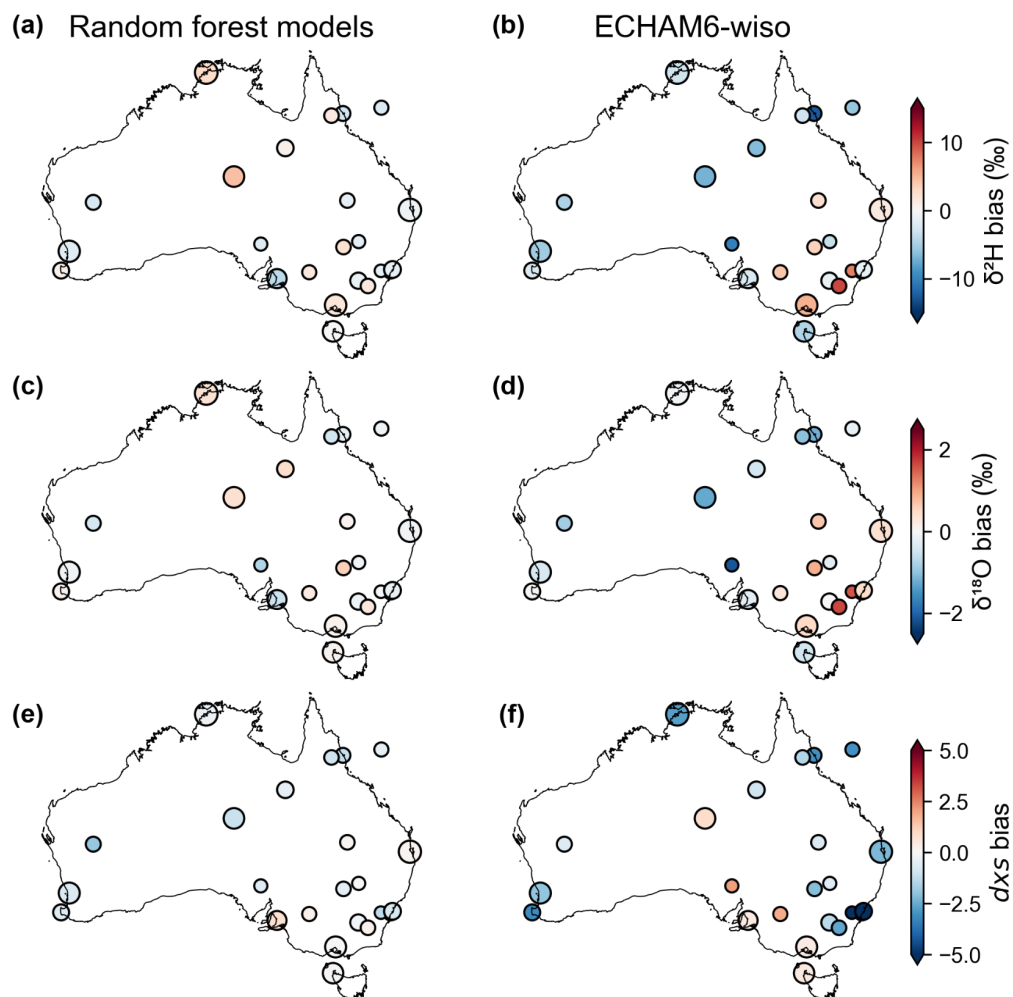
Figure S18: As per Fig. S17 but showing model bias relative to long-term observed annual means only in years included in both models (i.e., allowing direct comparison of the bias magnitudes). Note that the colour scales differ from Fig. S17.
