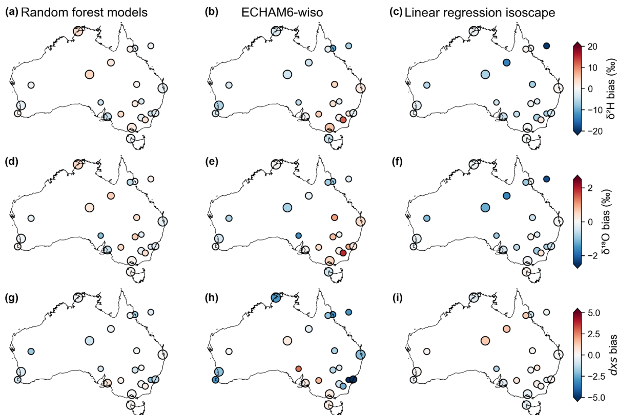
Figure S17: As per Fig. 11 but at each site showing the model's bias relative to observations in the long-term annual mean \delta^2\text{H}_\text{P} (a–c), \delta^{18}\text{O}_\text{P} (d–f) and dx_{\text{SP}} (g–i) at each site. Only showing sites with 5 or more years of monthly precipitation isotopic observations. The first column shows bias in the random forest models described in this paper (showing the mean of the 50 models created with unique random seeds); second column shows bias in ECHAM6-wiso nudged to ERA5; third column shows bias in the linear regression using geographical variables. Point size scales log-linearly with record length (in years).
