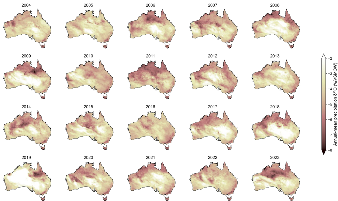
Figure 11: Precipitation amount-weighted annual mean \delta^{18}\text{O}_\text{P} values across Australia for the 20 most recent years of the random forest models trained over 1962–2023, using the reduced set of predictor variables (without weather objects).
