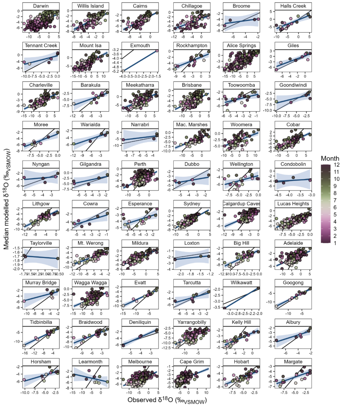
Figure 45: Crossplots comparing modelled and observed monthly \delta^{18}\text{O}_p values at the 60 sites across Australia with \delta^{18}\text{O}_p observations. For each site, \delta^{18}\text{O}_p values were predicted out of sample (i.e., that site's data was removed from the training dataset). Each point shows the mean of values predicted by 50 unique random forest models, each initiated with a different random seed. Sites are arranged by decreasing latitude, with the northern-most site (Darwin) in the top left corner and the southern-most site (Margate) in the bottom right corner. Site details are as per Table S1. In each panel, the thin black line shows the expected relationship if modelled \delta^{18}\text{O}_p values exactly matched observations (1:1). The blue line shows the linear relationship between the modelled and observed \delta^{18}\text{O}_p values, with the 95% confidence interval shown in the blue shading. Data points are coloured by month to highlight the seasonal cycle. Values are from the longer models trained over 1962–2023, using the reduced set of predictor variables (without weather objects).
