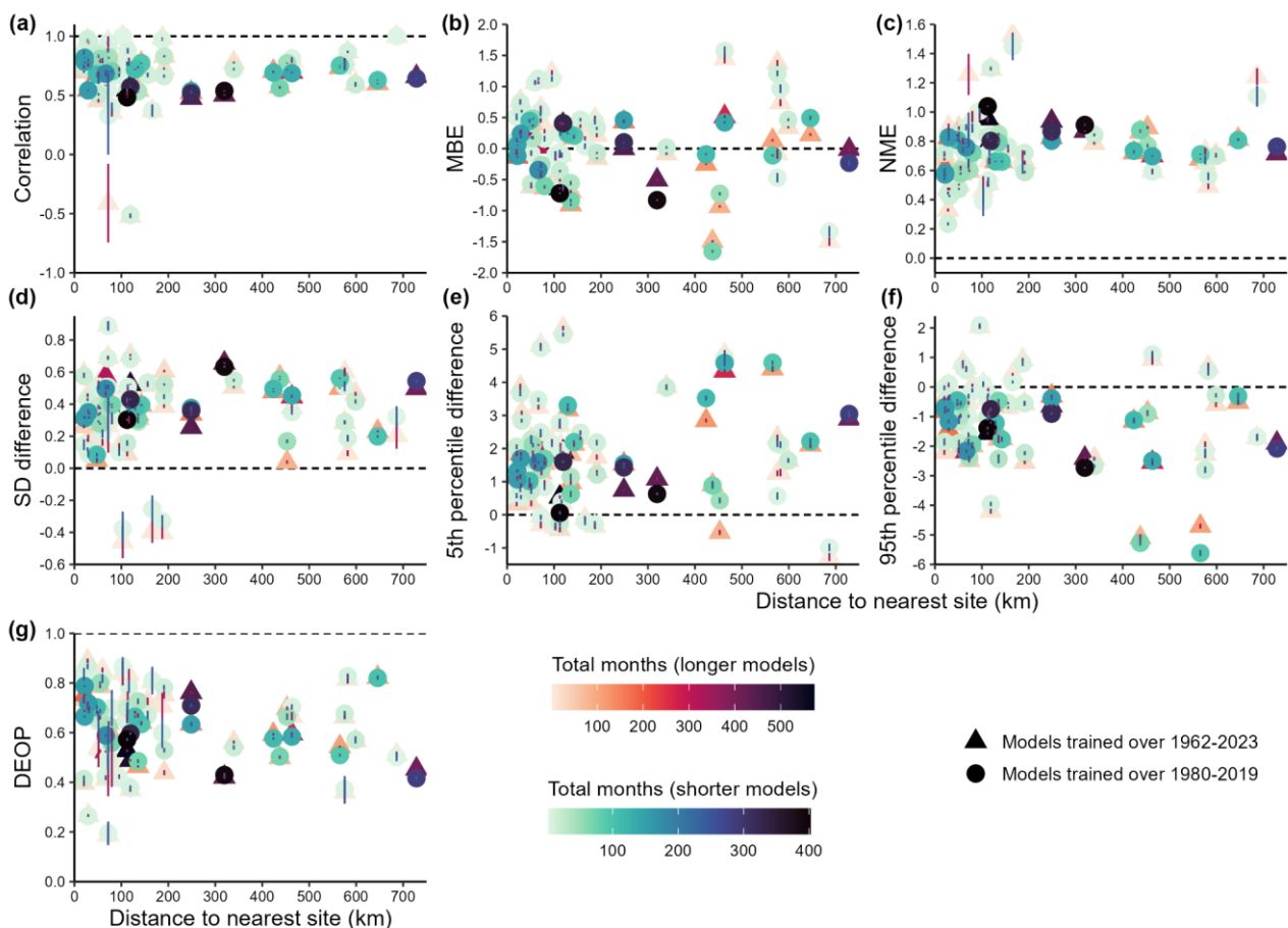
995 Figure 1: Crossplots summarising a suite of independent metrics describing out-of-sample random forest model skill 1000 in predicting spatial \delta^{18}\text{O}_p variability. Scores were calculated by removing one site from the training data (the ‘test site’), training a random forest model using the remaining data, then using that model to predict values for the excluded test site. This process was repeated 50 times for each site, each time initialising the random forest model with a different random 1005 seed. Each point shows the skill for a single site. Sites are plotted according to the distance to the nearest site included in the training dataset. Each site has two points on each crossplot: triangles show results for \delta^{18}\text{O}_p predicted using the longer models trained over 1962–2023 using the reduced set of predictor variables (without weather objects). Circles show results for \delta^{18}\text{O}_p predicted using models trained over 1980–2019 using the full set of predictor variables (including weather objects). Sites are coloured according to record length. The vertical line over each point shows \pm one standard deviation in that skill 1010 score across the 50 models. In all cases, the dashed black line shows the expected value if the modelled values perfectly matched observations. Panel (a) shows the Pearson correlation coefficient between the observed and modelled monthly \delta^{18}\text{O}_p values. Panel (b) shows the Mean Bias Error (MBE). Panel (c) shows the Normalised Mean Error (NME). Panel (d) shows the difference between the Standard Deviation (SD) of the observed and modelled values (following (Abramowitz et al., 2024), a positive value denotes modelled values have lower SD than observations). Panel (e) shows the difference in the 5th percentile of modelled versus observed values (a positive value denotes the 5th percentile of the modelled values has a positive bias relative to observations). Panel (f) shows the difference in the 95th percentile of modelled versus observed values (a negative value denotes the 95th percentile of the modelled values has a negative bias relative to observations). Panel (g) shows the density estimate overlap proportion (DEOP), which summarises the degree of overlap between density estimates calculated for the modelled and observed values (a value of 1 would indicate perfect overlap; 0 would indicate no overlap). See Section 2.2.1 or Table S4 in Abramowitz et al. (2024) for skill metric definitions.
