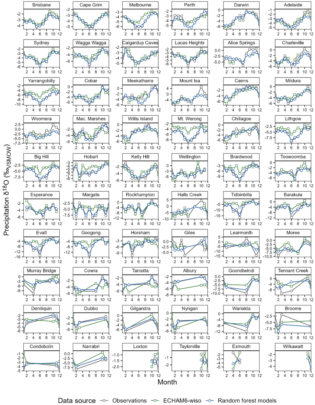
Figure 56: Average seasonal cycle of \delta^{18}\text{O}_\text{p} at 60 sites across Australia, in observations (grey circles); the random forest models described in this paper (blue diamonds); and the ECHAM6-wiso simulation nudged to the ERA5 reanalysis (see Methods; green squares). Seasonal cycles are calculated from \delta^{18}\text{O}_\text{p} values in the interval overlapped by all three data sources (1979–2021), and only include months with observations present in all three data sources. In the case of the random forest-predicted \delta^{18}\text{O}_\text{p} , values are from the longer models trained over 1962–2023, using the reduced set of predictor variables (without weather objects), and show the mean of the 50 models created with unique random seeds. Sites are arranged by decreasing number of observations. Brisbane (top left) has the most observations ( n = 500 ); Wilkawatt and Exmouth (bottom right) have the equal fewest observations ( n = 3 ).
