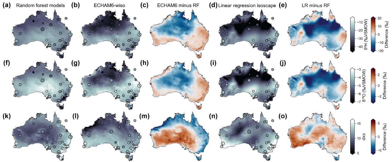
1225 Figure 413: Long-term annual mean precipitation isotopic variability across the Australian continent ('time-mean isoscapes'). Panel (a) shows long-term (1962–2023) annual-mean precipitation amount-weighted \delta^2\text{H}_p as calculated from the random forest models described in this paper (showing the mean of the 50 models created with unique random seeds). Panel (b) shows long-term (1979–2021) annual-mean precipitation amount-weighted \delta^2\text{H}_p as simulated by ECHAM6-wiso nudged to ERA5 (Cauquoin and Werner, 2021). Panel (c) shows the difference between climatological \delta^2\text{H}_p from ECHAM6-wiso and the random forest models (i.e., panel (b) minus panel (a)). Panel (d) shows long-term (1962–2014) annual-mean precipitation amount-weighted \delta^2\text{H}_p as estimated by linear regression using geographical variables (Hollins et al., 2018). Panel (e) shows the difference between climatological \delta^2\text{H}_p from the linear regression and the random forest models (i.e., panel (d) minus panel (a)). Panels (f–j) are as per panels (a–e) but for \delta^{18}\text{O}_p . Panels (k–o) are as per panels (a–e) but for d_{xsp} . Note that the isoscapes from Hollins et al. (2018) were calculated using data spanning 1962–2014, which exceeds the total coverage of the ECHAM6-wiso simulation. As we could not average across matching time periods for all three data sources, we show annual means across each dataset's entire coverage interval to provide the most representative long-term isoscapes. Points show the long-term annual mean precipitation isotopic values at each site with 2 or more years of observations (see Section 2.4 for details). Point sizes scale log-linearly with record length (in years).
