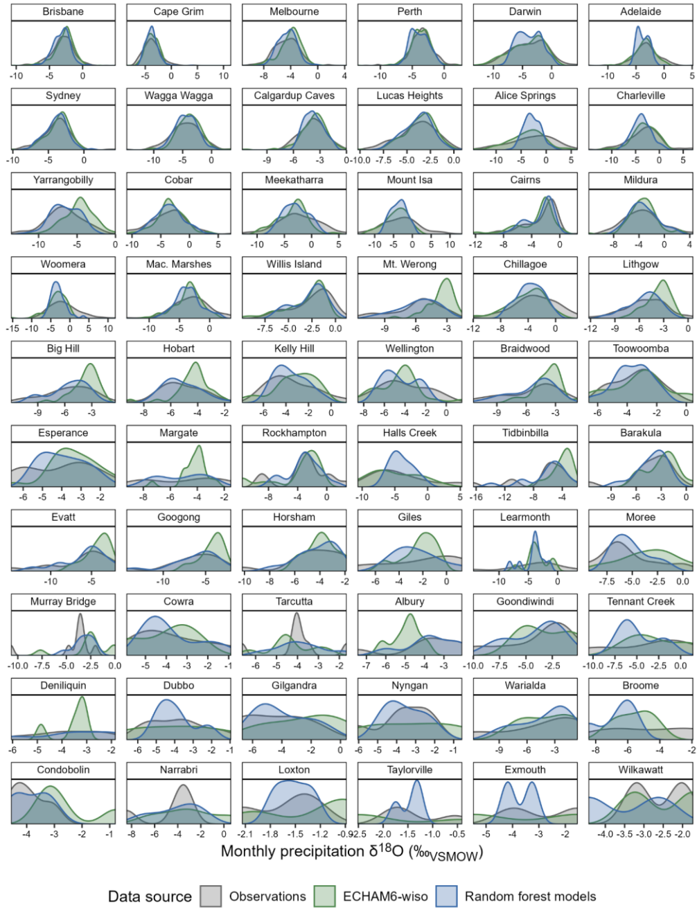
1115 Figure 67: Density plots comparing the distributions of monthly \delta^{18}\text{O}_p values at 60 sites across Australia, from observations (grey); the random forest models described in this paper (blue); and the ECHAM6-wiso simulation nudged to the ERA5 reanalysis (see Methods; green). Density curves are calculated from \delta^{18}\text{O}_p values in the interval overlapped by all three data sources (1979–2021), and only including months with observations (i.e., curves are constructed with \delta^{18}\text{O}_p values from exactly the same months). In the case of the 1120 random forest-predicted \delta^{18}\text{O}_p , values are from the longer models trained over 1962–2023, using the reduced set of predictor variables (without weather objects), and show the mean of the 50 models created with unique random seeds. Sites are arranged by decreasing number of observations across 1979–2021. Brisbane (top left) has the most observations ( n = 500 ); Wilkawatt and Exmouth (bottom right) have the equal fewest observations ( n = 3 ).
