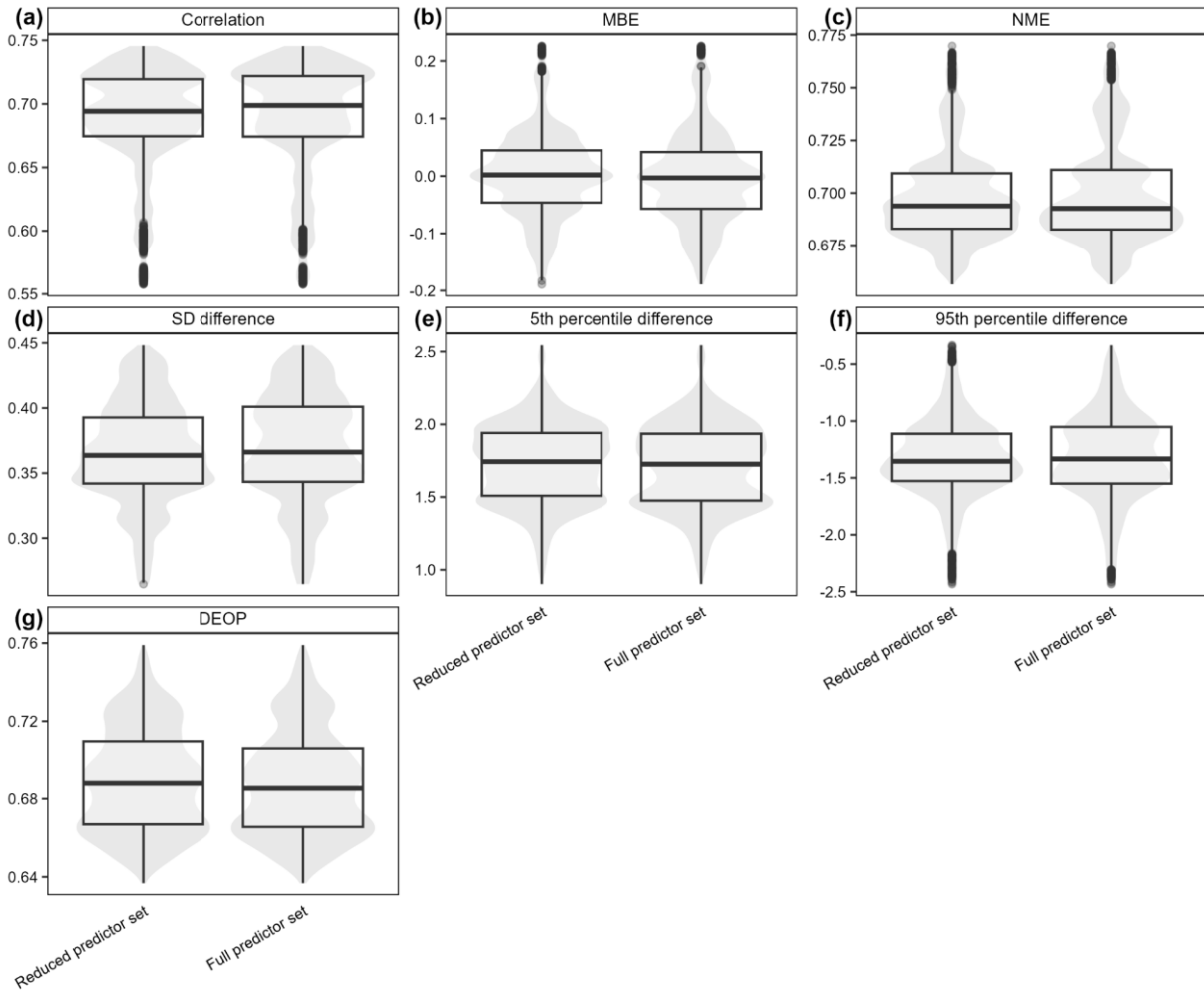
1035 Figure 3: Violin-and-boxplots (‘voxplots’) summarising a suite of independent metrics describing model skill in predicting out-of-sample temporal \delta^{18}\text{O}_\text{p} variability (across all sites). Scores were calculated by removing a random 10% of all training data, predicting the missing values, then assessing the model’s skill in retrieving the held-out data. This process was repeated such that all training data were tested out-of-sample. Additionally, each random forest model was calculated 50 times, each time with a different random seed. These two iterative processes comprise the distributions. In each 1040 panel, the left voxplot shows results for monthly \delta^{18}\text{O}_\text{p} predicted using models trained over 1962–2023, using the reduced set of predictor variables (without weather objects). The right voxplot shows results for monthly \delta^{18}\text{O}_\text{p} predicted using models trained over 1980–2019, using the full set of predictor variables (including weather objects). Skill metrics across panels (a– g) are all as per Fig. 1.
