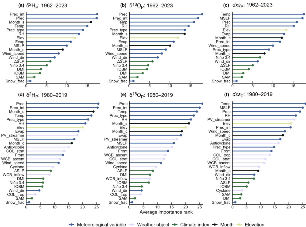
Figure 79: Average importance rank of each predictor variable with respect to the random forest models' predictive performance, calculated using the 'permutation' method. The panels show the overall rank of each variable's relative importance in predicting spatio-temporal precipitation isotopic variability across the Australian continent. Ranks are the average for that variable across 50 random forest models, each created with a different random seed. The least important variable for a predictor model receives a rank of 1; the most important variable receives a rank equal to the number of variables included. So, the most important variables for the model are shown at the top of each panel; the least important at the bottom. Predictors are coloured according to the variable type: blue for meteorological variables, lavender for weather objects, forest green for climate indices (representing remote dynamical drivers), black for month of the year, and lime green for elevation. Panel (a) shows results for the \delta^2\text{H}_\text{P} models trained over 1962–2023, using the reduced set of predictor variables (without weather objects). Panel (b) is as per panel (a) but for \delta^{18}\text{O}_\text{P} . Panel (c) is as per panel (a) but for \text{dxs}_\text{P} . Panels (d–f) are as per panels (a–c) but for the models trained over 1980–2019, using the full set of predictor variables (including weather objects). Variable names and descriptions are as per Table S2.
