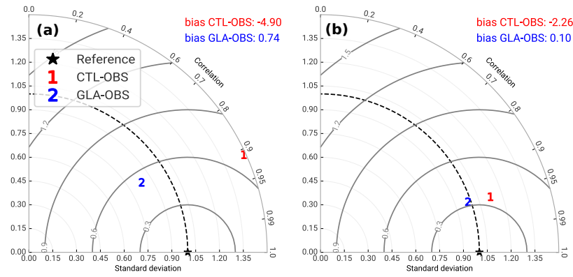
Figure 5. Taylor diagrams of hourly snow temperature of the modelled snowpack interpolated at the sensor depth for ecLand control experiment (CTL) and ecLand with the new glacier parameterisation (GLA) using in situ forcing (CTL-OBS and GLA-OBS) relative to observations at the PROMICE stations, aggregated at the (a) upper and (b) accumulation sites for the entire period of available observations at each site. Each panel reports the bias computed over all sites for the entire period for the different experiments. See Sect. 2.4.1 for details on the different experiment setups.
