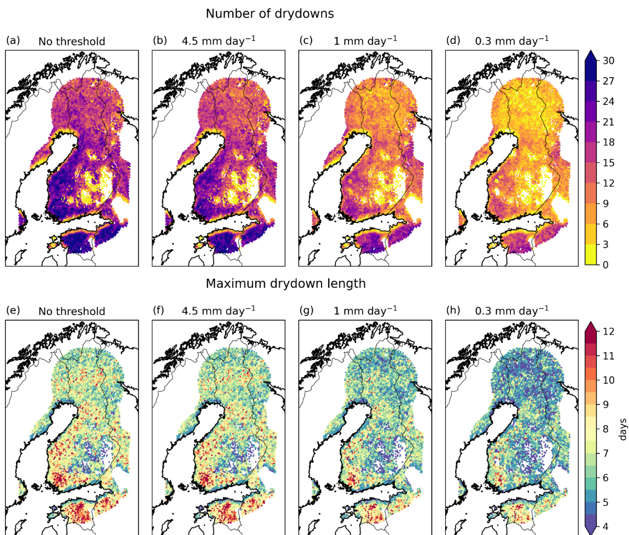
Figure S2. The number of drydowns and the maximum drydown length using different P thresholds when identifying drydowns.
