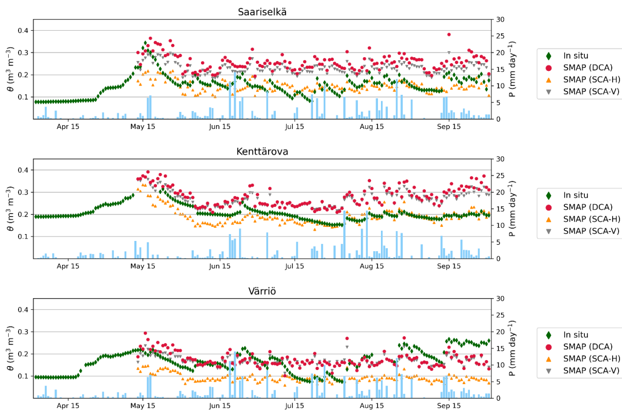
Figure S1. Timeseries of SM and radar-based P measurements in Saariselkä, Kenttäröva, and Värriö.
