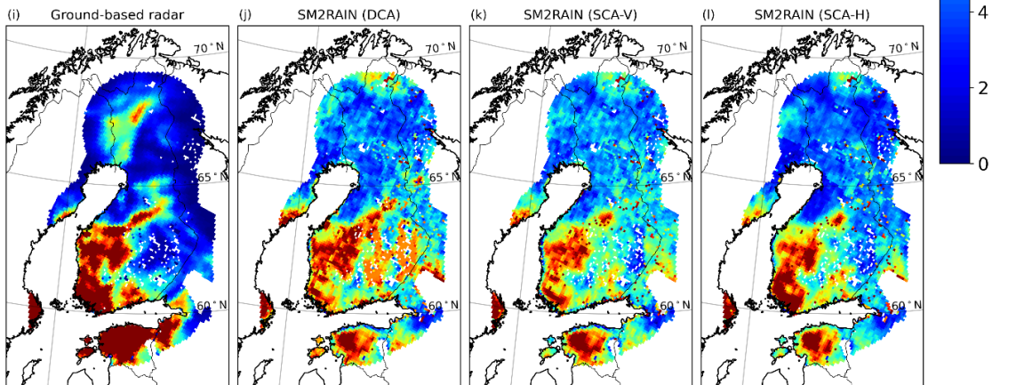
Figure 7. 6-day accumulated P based on radar data and SM2RAIN algorithm for three selected periods.
