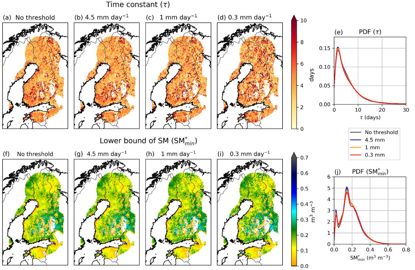
Figure 9. The median time constant and the median lower bound of SM using different P thresholds when identifying drydowns.
