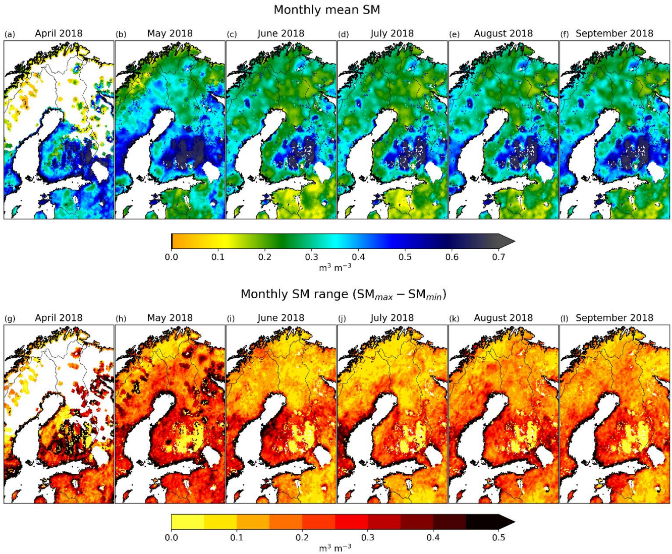
270 Figure 4. (a-f) Monthly mean SM and (g-l) monthly SM range in 2018.
