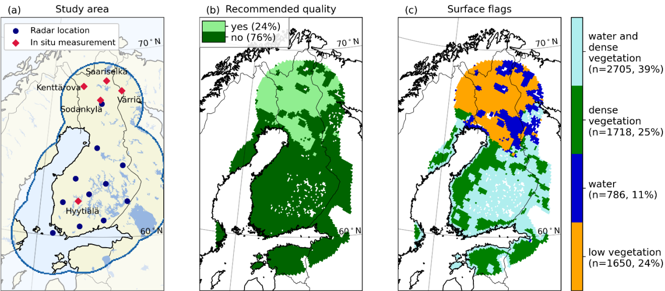
Figure 2. (a) The study area and the locations of the ground-based weather radars and in situ measurements. (b) The quality retrieval flags for SMAP. (c) The surface flags for SMAP. The percentages indicate the fraction of grid cells included in the category.
