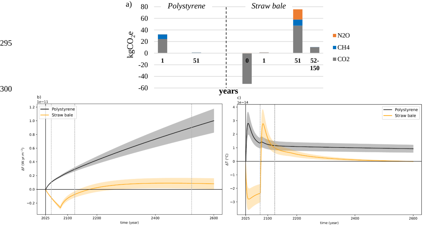
Figure 4. a) Emission profile of 1m² of thermal insulators - Polystyrene and Straw bale – having a thermal resistance of 7 m² K W⁻¹ during 50 years. CO₂, CH₄ and N₂O are emitted (see inventories in S7). b) ΔF and c) ΔT temporal profiles of these two products over 575 years. Dotted grey lines represent H given by IPCC leading to ΔF 20 , ΔF 100 , ΔF 500 (b) ; ΔT 50 , ΔT 100 (c).
