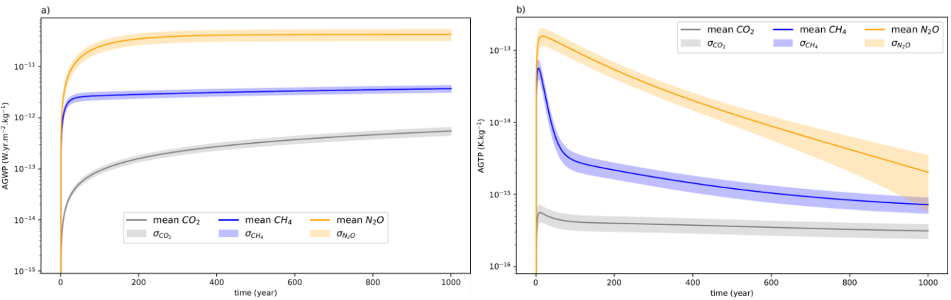
Figure 1. a) AGWP and b) AGTP profiles in logarithmic scale from present-day (H = 0 year) to very long-term perspective (H = 1000 years) after emissions of 1kg CO 2 , 1kg CH 4 and 1kg N 2 O. Uncertainty ranges are computed by varying all parameters listed in Table 1.
