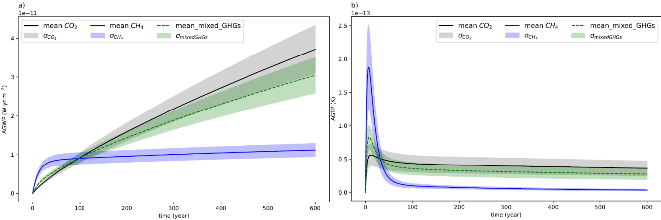
280 Figure 2. a) AGWP and b) AGTP profiles for three pulse emissions having the same GWP_{100} = 100 \text{ kgCO}_2\text{e} .
