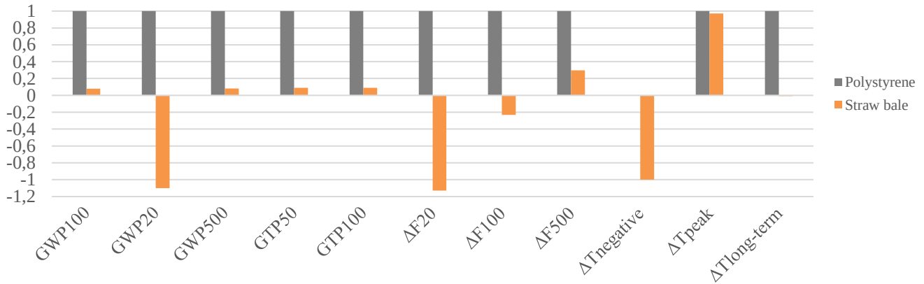
Figure 5. Relative climate change results for Polystyrene and Straw bale according to common relative metrics – GWP 20 , GWP 100 , GWP 500 , GTP 50 , GTP 100 - and suggested metrics in this article: \Delta F_{20} , \Delta F_{100} , \Delta F_{500} , \Delta T_{\text{negative}} , \Delta T_{\text{peak}} , \Delta T_{\text{long-term}} . Absolute values are presented in S8. Pulse emissions occurring outside the timeline [ t_0 , H] are not considered.
