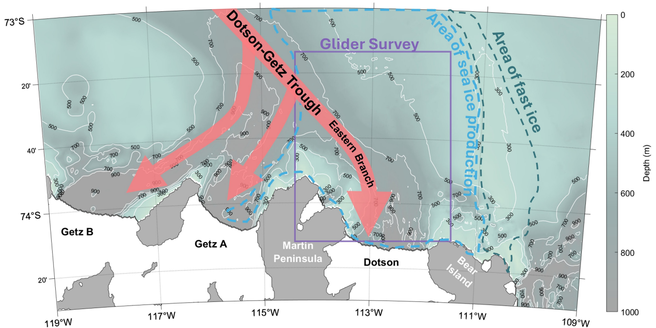
Figure 1. Map of the study region within the Amundsen Sea polynya. Arrows indicate the pathway of mCDW following the Dotson-Getz Trough (Wåhlin et al., 2010). Contours show BedMachine v3 bathymetry (Morlighem, 2022). The purple box indicates the boundaries of the glider transect map in Fig. 3c. The dashed blue line represents the area of sea ice production and the dashed green line shows the location of permanent fast ice, both shown in Figure 3 of Ohshima et al. (2016).
