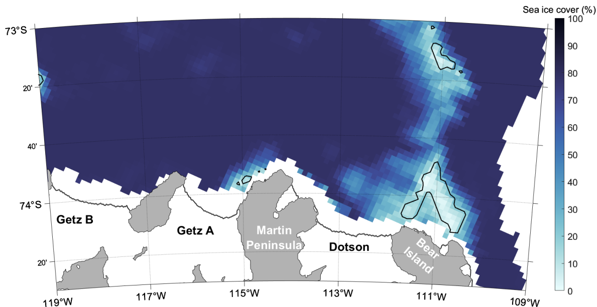
Figure 9. Sea ice cover from AMSR2 (%) for 18 July 2021 in the southern Amundsen Sea polynya . The areas with a light blue colour and areas within the black lines have less than 15% sea ice cover. Ice imagery from AMSR2 . White areas indicate a lack of imagery data .
