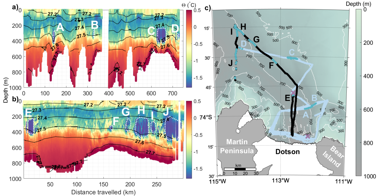
Figure 3. Lenses identified in glider transects. \Theta is shown for depth and distance travelled by a) SG579 and b) SG510. Black contours show potential density ( \text{kg m}^{-3} ). Cold lenses (A-J) are outlined in white dashes. c) The location of the glider transects (blue for SG579 and black for SG510) and the lenses (green). The purple crosses depict where each respective glider transect starts. Bathymetry is from BedMachine v3 (Morlighem, 2022) and isobaths are plotted in white.
