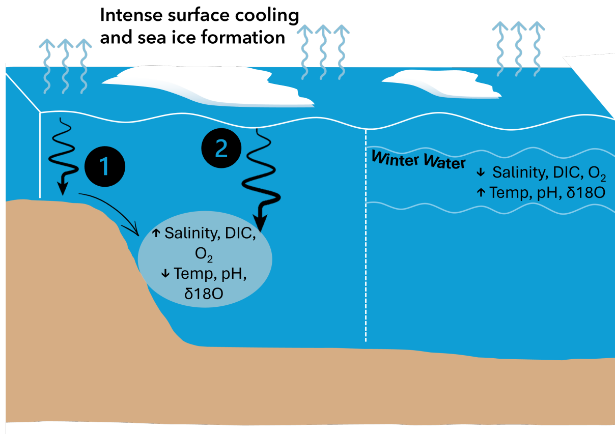
Figure 8. Schematic depicting (left hand side) the two possible-hypothesised formation processes-mechanisms of the lenses on-the-left and their properties. The numbers reference the formation theory-mechanism with (1) formation in shallow water due to sea ice formation and spilling into deeper water and (2) local chimneys of convective mixing. The right hand side depicts the properties of the overlying WW relative to the lenses.
