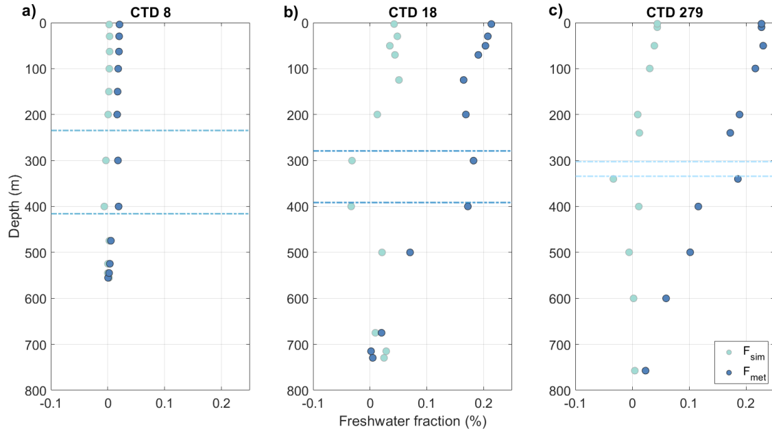
Figure 6. Vertical profiles of freshwater fractions from meteoric (blue) and sea ice melt (green) sources derived from \delta\text{D} - \delta^{18}\text{O} and S_A measurements for the three CTD casts with lenses. The horizontal blue dashed lines indicate the locations of the lenses with colours corresponding to CTD profile following Figs 4 and 5.
