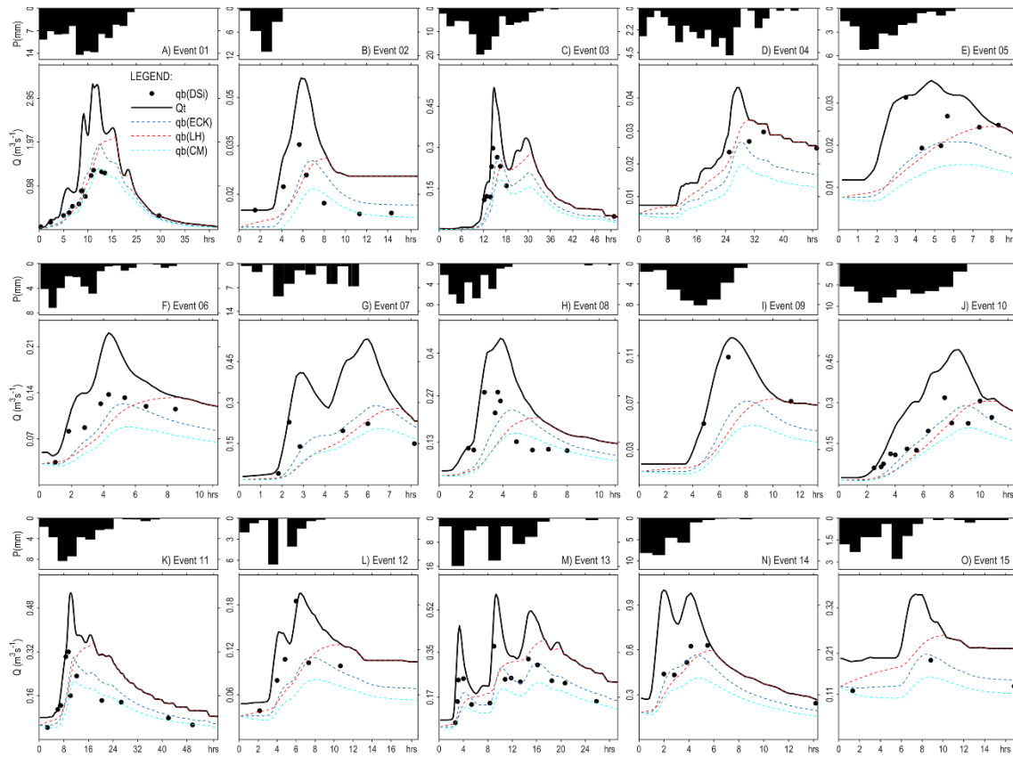
Figure 2. Comparison of baseflow separation techniques on 15 events in the Arvorezinha catchment (Brazil): total
