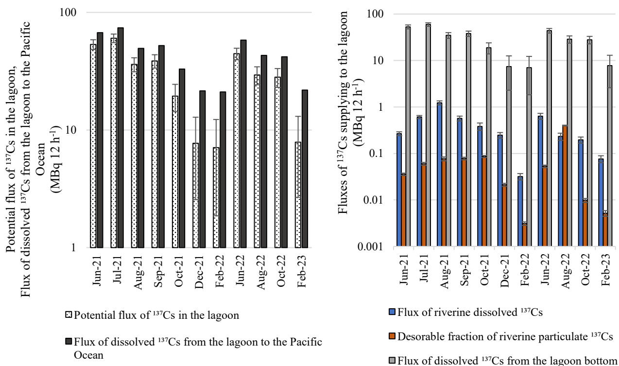
350 Figure 8: Potential fluxes of dissolved ^{137}\text{Cs} supplied to Matsukawa-ura lagoon and fluxes of dissolved ^{137}\text{Cs} from the lagoon to the Pacific Ocean (a). Fluxes of dissolved ^{137}\text{Cs} supplied to the lagoon from the rivers, desorbed from riverine particles and the lagoon bottom in the lagoon (b). Black bars represent the measurement error of ^{137}\text{Cs} .
