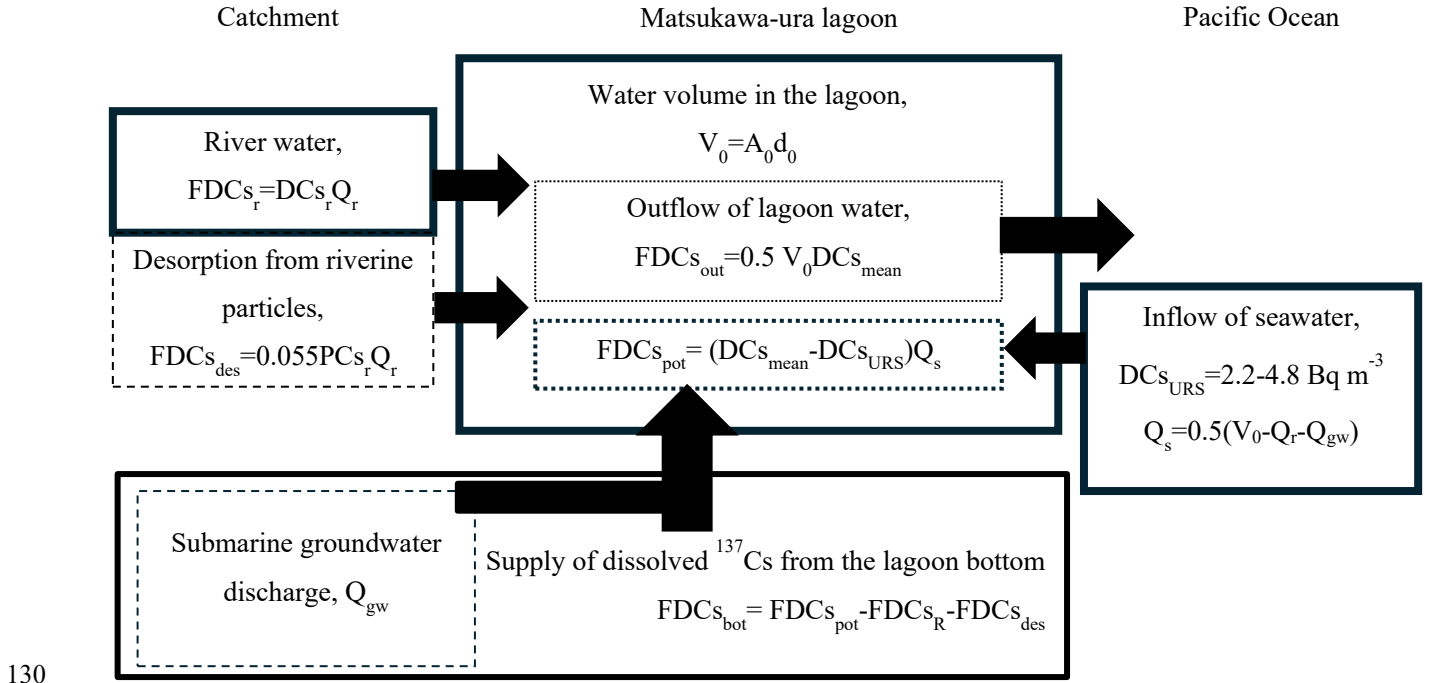
Figure 2: Schematic illustration of the box-model for water and dissolved ^{137}\text{Cs} in Matsukawa-ura Lagoon. Half of the lagoon water volume was assumed to be exchanged with coastal seawater during each tidal cycle under spring tide conditions (Kohata et al., 2003), and 5.5% of riverine particulate ^{137}\text{Cs} was assumed to be converted to dissolved ^{137}\text{Cs} through desorption after entering the lagoon (Takata et al., 2021).
