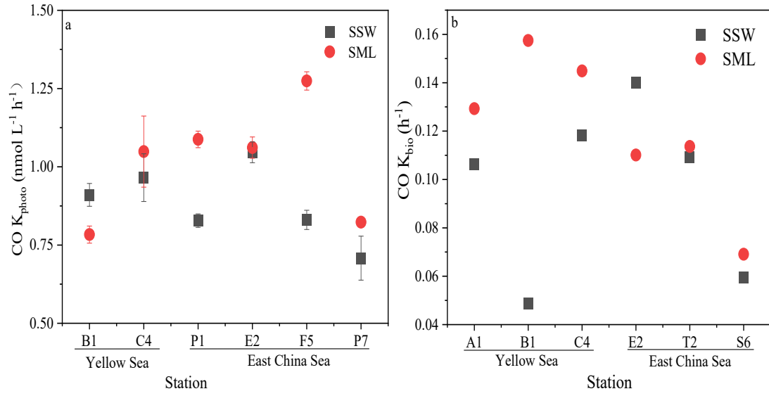
Fig. 4 Variations in photochemical CO production rate of CO ( \text{K}_{\text{photo}} ) in the SML (red) and the SSW (black) (a)). Variations in microbial consumption rate constants of CO ( \text{K}_{\text{bio}} ) in the SML (red) and the SSW (black). Data are presented as mean values and error bars represent the standard deviation of duplicate samples.
