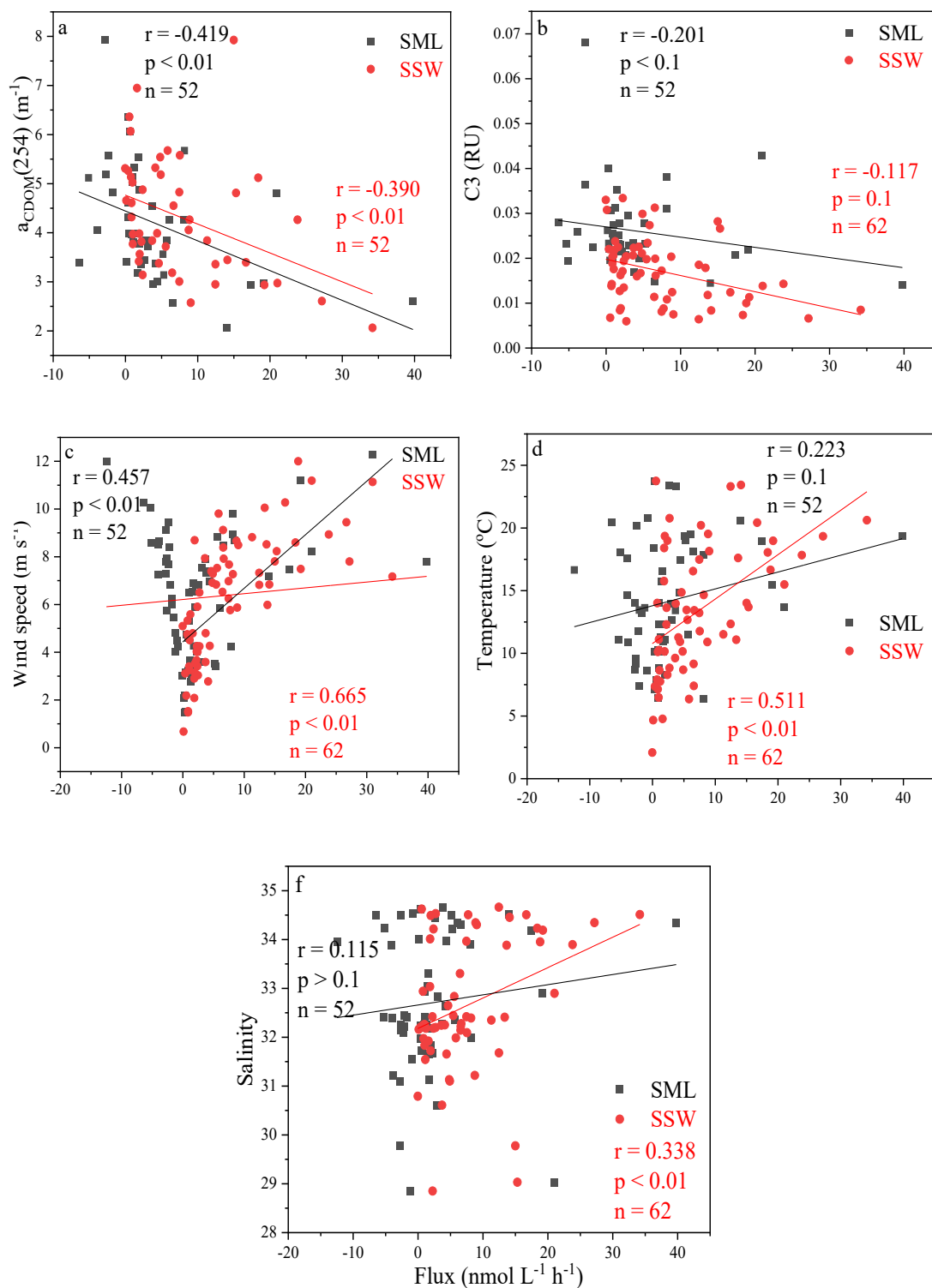
Fig. 5 Correlations between the instantaneous sea-to-air fluxes of CO (Flux) in the SSW and the SML with a_{\text{CDOM}}(254) , marine humic-like C3, wind speeds, temperature, and salinity in the East China Sea and the Yellow Sea during winter.
