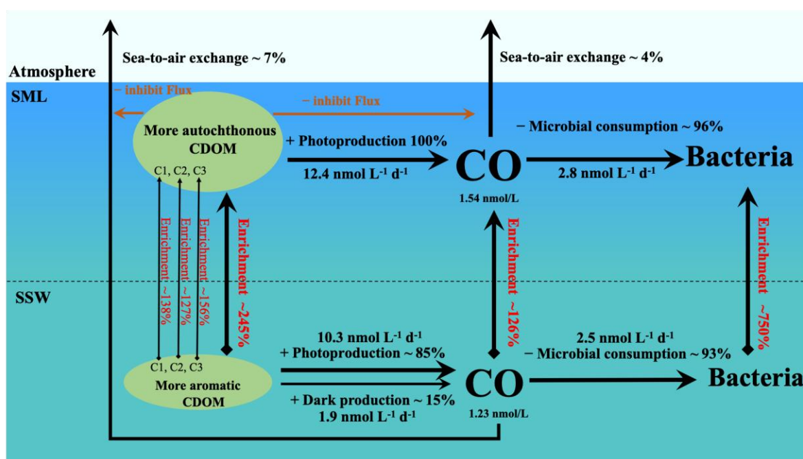
3 Fig. 6 Budget model of CO transformation in the SML and the SSW in the eastern 4 marginal seas of China during winter. (Bacterial enrichment was calculated by Sun et 5 al., 2020).
