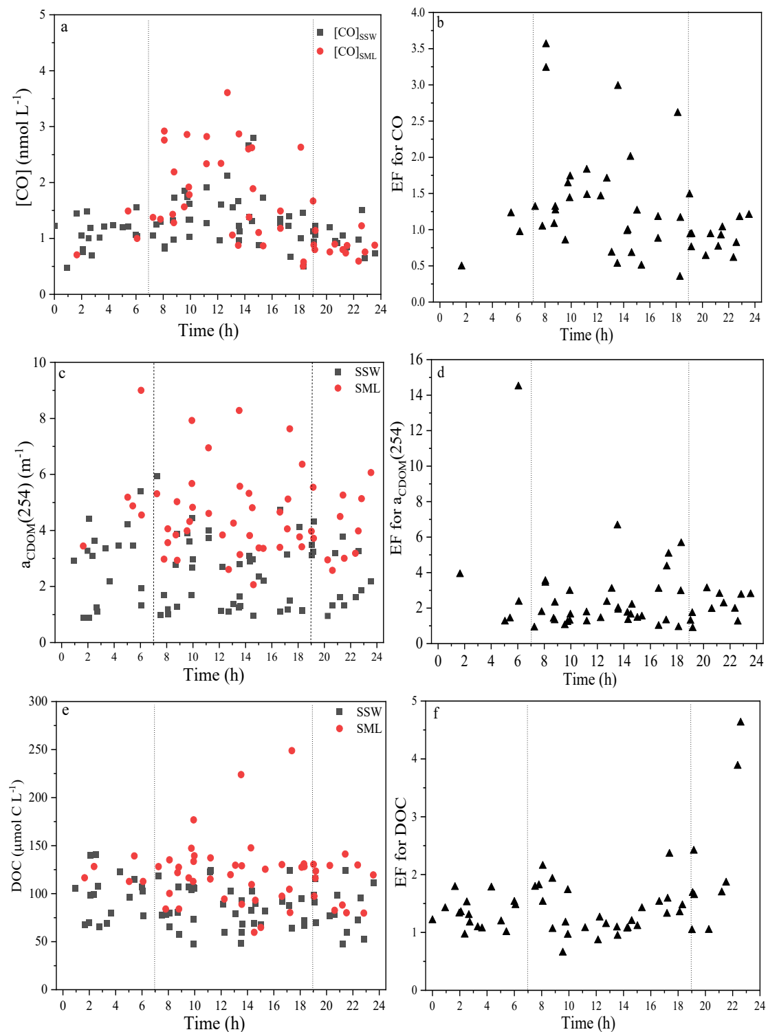
Fig. 3 Variations in the [\text{CO}]_{\text{SML}} , [\text{CO}]_{\text{SSW}} , a_{\text{CDOM}}(254) , and DOC, EFs of [\text{CO}] , a_{\text{CDOM}}(254) , and DOC with the sampling time at each station.
