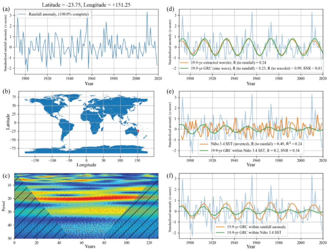
Figure 9. Comparison of contributions of the relative strength of the 19.9-year cycle in rainfall at a selected site in Australia and the Niño 3.4 SST. (a) Normalised (z-score) rainfall anomaly for the site, complete time series with no infilling. (b) Site location on a global map. (c) The wavelet spectrum of annual rainfall. (d) The rainfall anomaly with the 19.9-year cycle extracted by wavelet analysis (orange), and the fixed 19.9-year GRC (green). (e) The rainfall anomaly shown with the Niño 3.4 SST time series (orange) scaled by linear regression to visualise contribution to rainfall, and the 19.9-year component of the Niño 3.4 SST time series (green). (f) the rainfall anomaly with the 19.9-year cycle extracted from rainfall (orange) and the Niño 3.4 SST time series (green). Though the two cycles are mostly in phase, the GRC in rainfall has a much higher SNR (0.81 versus 0.34) as well a consistent amplitude and period.
