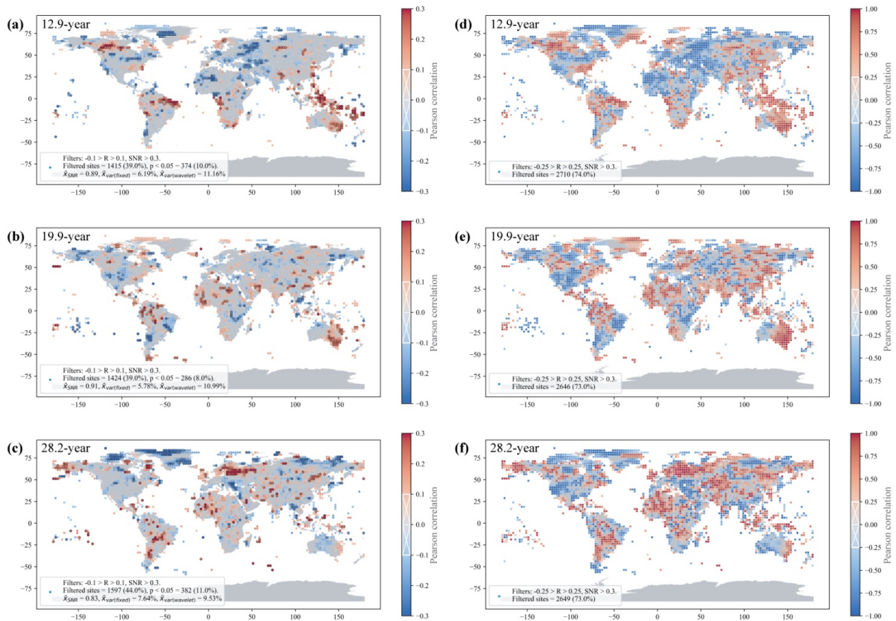
Figure 6. Global distribution of the 12.9-, 19.9- and 28.2-year GRCs modelled as sine waves with phase offsets matching the Australasian region. (a-c) The Pearson correlation coefficient (R) of the sine wave to rainfall anomaly at each site with significant sites ( p < 0.05 ) circled in black, and display threshold of 1% of annual rainfall variance calculated by coefficient of determination ( R^2 ). (d-f) The Pearson correlation coefficient (R) of the GRC sine wave to the corresponding extracted wavelet with a threshold of 0.25. Both methods show clustering in the same regions for each cycle. Comparison to the wavelet allows a broader picture of the cycle influence by controlling the masking effect of high frequency noise.
