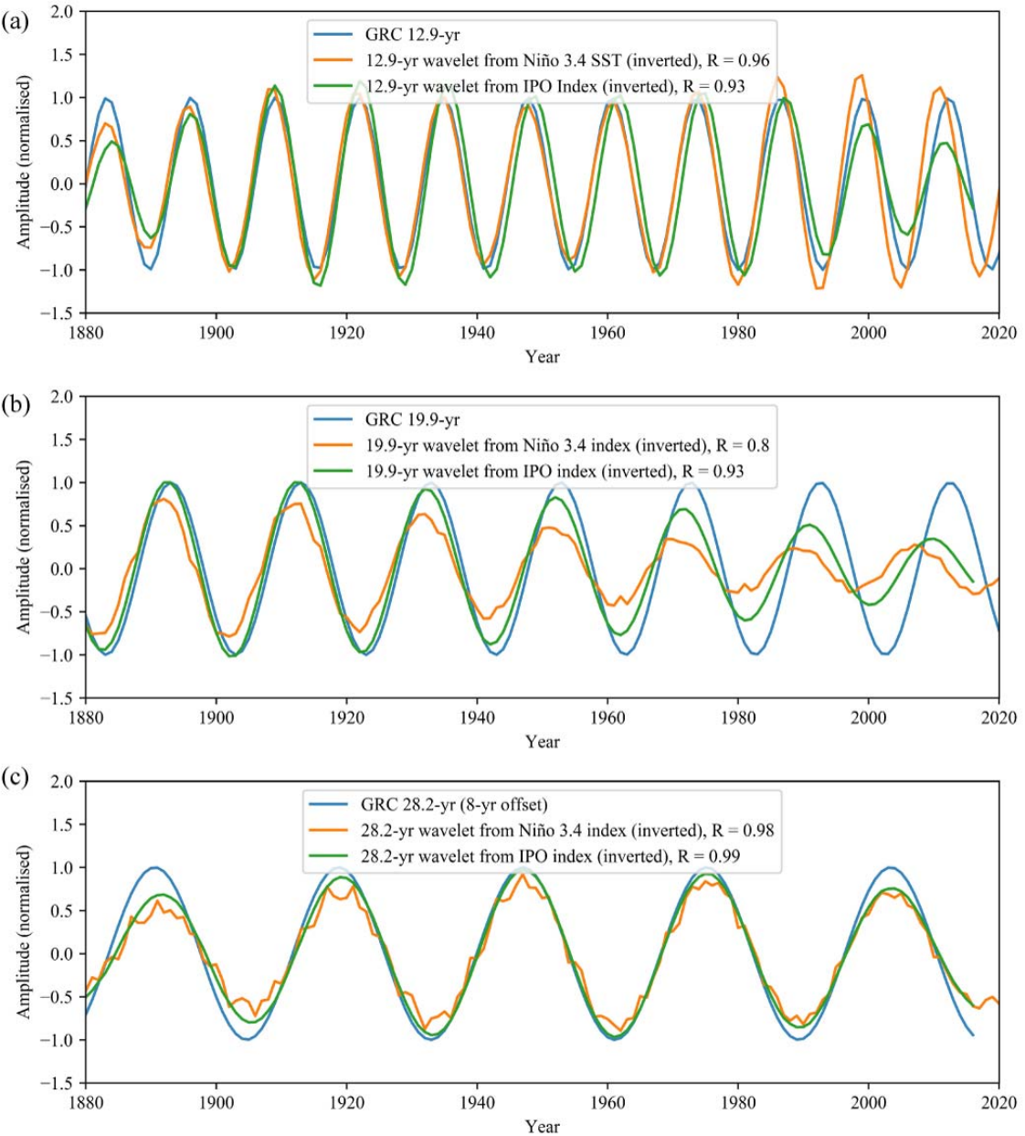
380 Figure 8. Comparison of the fixed 12.9-, 19.9-, and 28.2-year GRCs with the extracted cycle from wavelet analysis of the major climate modes. (a) Strong phase alignment can be seen between the 12.9-year GRC, Niño 3.4 and IPO ( R > 0.9 ). (b) The 19.9-year GRC aligns well
