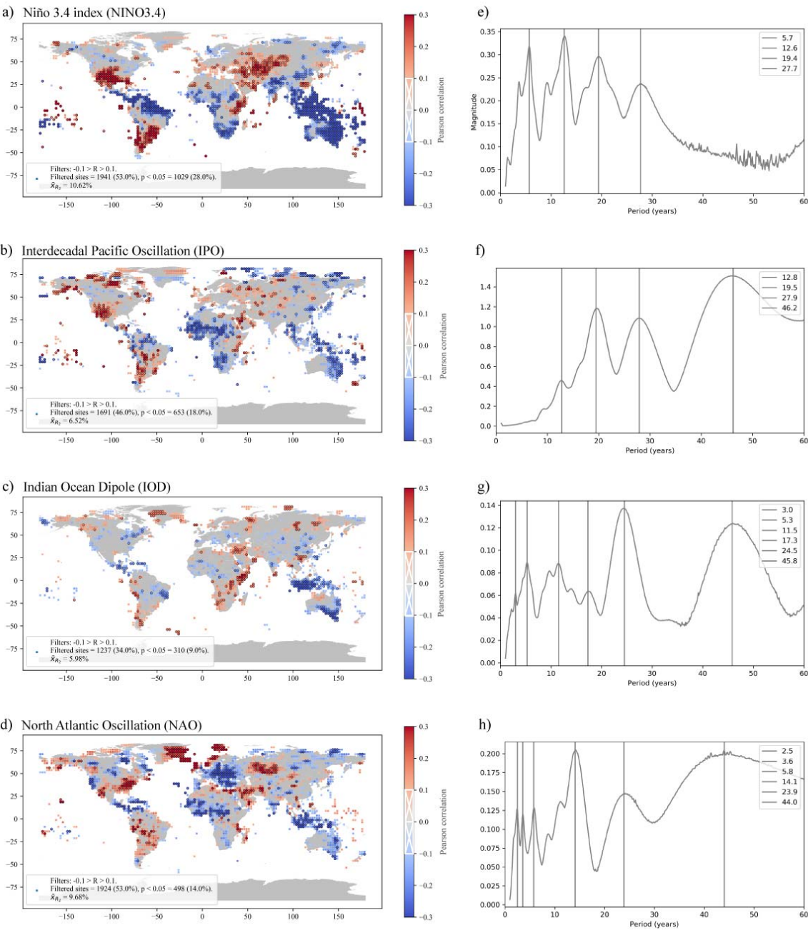
Figure 7. Geographical regions of influence of the major climate modes and corresponding cycles extracted from the wavelet GMPS. Left panels show the Pearson correlation (R) between rainfall and the relevant climate mode where it is over 0.1. Sites where the correlation is
