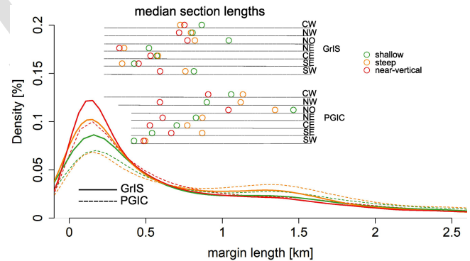
Figure 10. Density of individual connected margin sections according to their morphology, with shallow (green), steep (orange) and near vertical (red) margin sections. Data points longer than 2.5 km are not shown. Circles show median lengths across all margin sections for each subregion on both GrIS and PGIC.
