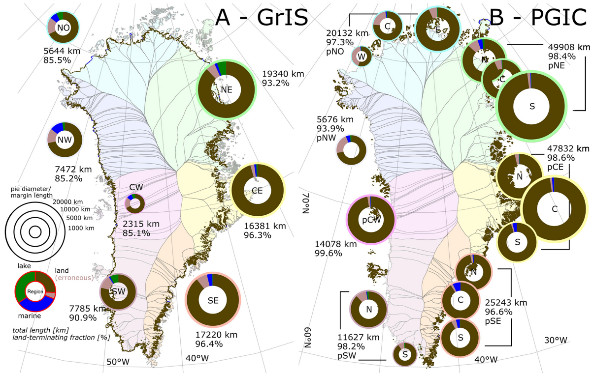
Figure 3. Margin lengths and respective land-, marine- and lake-terminating fractions for the GrIS (A) and PGIC (B). The numbers adjacent to the pie plots refer to total length and relative fraction of the land-terminating margin. Note that for PGIC the lengths are shown separately for subsections of the pNO, pNE, pCE, pSE and pSW regions, corresponding to data shown in Table S3, to avoid excessive size of pies (for pNE, pCE, pSE) and due to the disconnected nature of ice masses (pNO, pSW). Values of individual subbasins for the GrIS regions for PGICs are shown in Table S3.
