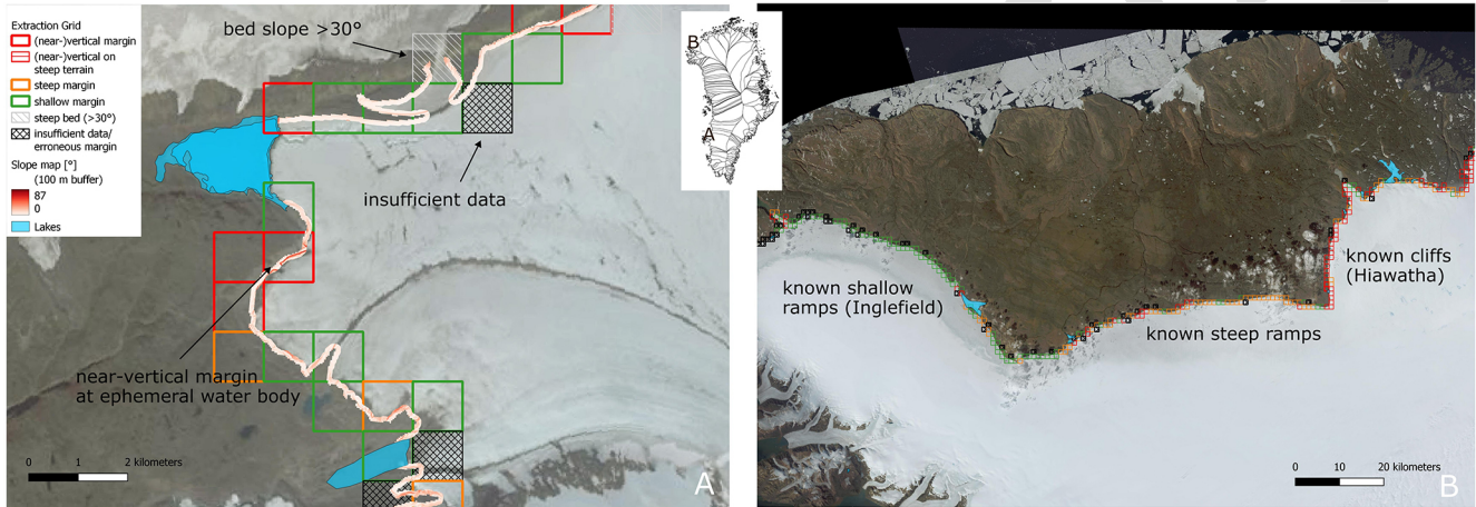
Figure 8. Examples of identified predominant margin morphologies in southwest (A, catchment 4) and northwest Greenland (B, catchment 176).
