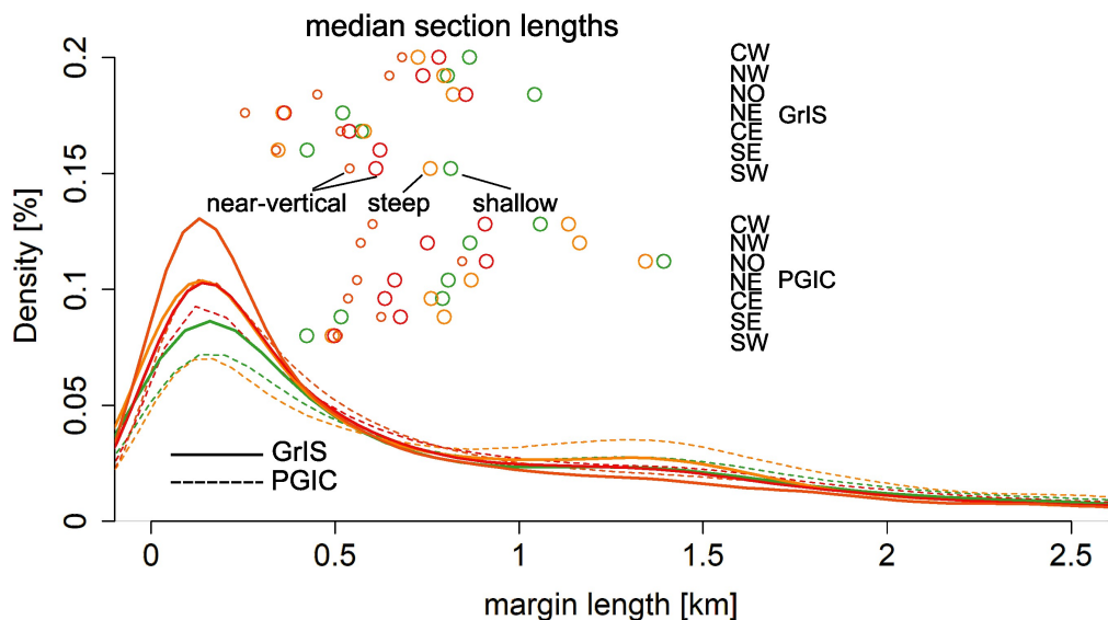
Figure 10. Density of individual connected margin sections according to their morphology, with shallow (green), steep (light orange), near vertical (red) and near-vertical on steep terrain (dark orange) margin sections. Data points longer than 2.5 km are not shown. Circles show median lengths across all margin sections for each subregion on both GrIS and PGIC.
