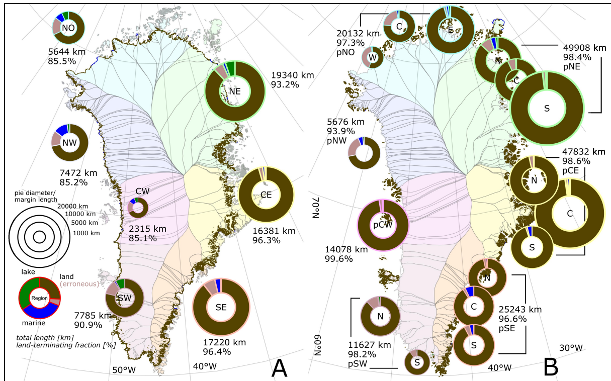
Figure 3. Marginal lengths and respective land-, marine- and lake-terminating fractions for the GrIS (A) and PGIC (B). The numbers adjacent to the pie plots refer to total length and relative fraction of the land-terminating margin. Note that for PGIC the lengths are shown separately for subsections of the pNO, pNE, pCE, pSE and pSW regions, corresponding to data shown in Table S3, to avoid excessive size of pies (for pNE, pCE, pSE) and due to the disconnected nature of ice masses (pNO, pSW). Values of individual subbasins for the GrIS regions for PGICs are shown in Table S3.
