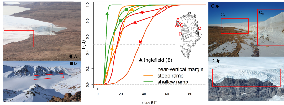
Figure 7. Cumulative distribution functions for selected margin sections, identifying near-vertical cliffs (red), steep ramps (orange) and shallow ramps (green). Symbols refer to regions where margin types were sampled, shown in the four photos. Horizontal dashed lines are the 50 th and 85 th quantile. Red squares in the photos denote the approximate margin areas selected. Locations A and C are at the Nunatarssuaq ice cap (Abermann et al., 2020), B is Freya Glacier, and D is located in West Greenland (Abermann et al., 2023, photo: Fauland/Wally). Locations in Inglefield Land are documented in Kjær et al. (2018) and Esenther et al. (2023).
