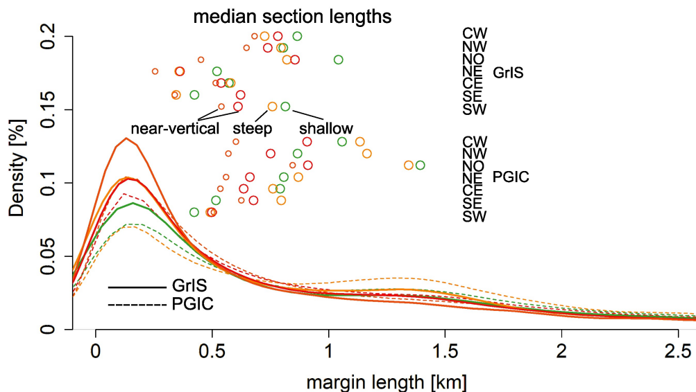
Figure 10. Density of individual connected margin sections according to their morphology, with shallow (green), steep (light orange), near vertical (red) and near-vertical on steep terrain (dark orange) margin sections. Data points longer than 2.5 km are not shown. Circles show median lengths across all margin sections for each subregion on both GrIS and PGIC.
