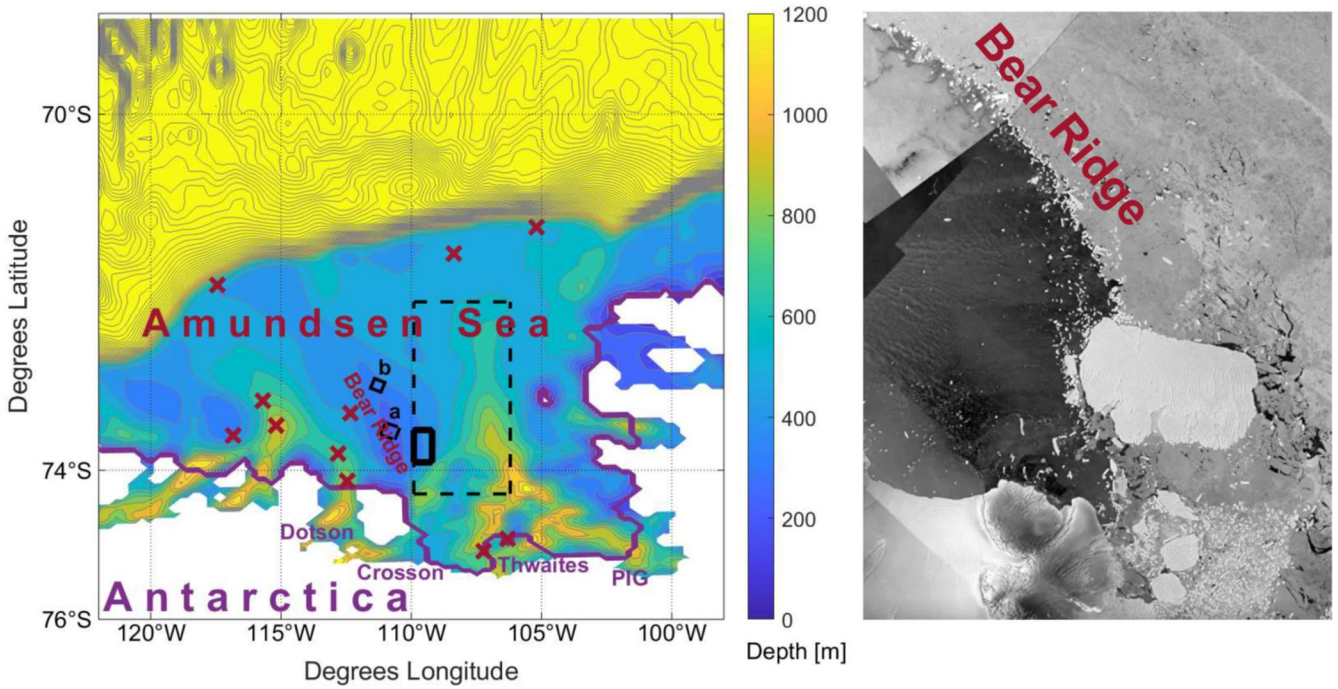
Figure 1: Left: Amundsen Sea and Bear Ridge topography [m] based on the BedMachine Antarctica dataset (Morlighem et al., 2020) and re-gridded on the model configuration grid. Gray contours are spaced 80 m apart. Thin solid black contours delimit the bounds of boxes a and b in Figure 2, indicating the sites of observed iceberg scours in Section 2.1 with magenta labels matching boxes a and b in Figure 2. Dark red crosses mark the locations of sediment samples analysed in Section 2.2. The thick purple line shows the ice shelf edge, with major ice shelves labelled: Dotson, Crosson, Thwaites, and Pine Island Glacier (PIG). Thick solid (thin dashed) black lines show the boundaries of the boxes where icebergs are released in the SHORT (LONG) simulations. Right: Copernicus Sentinel-1 SAR (synthetic aperture radar) image from 12 February 2022 over Bear Ridge with white shades indicating the presence of icebergs and sea-ice.
