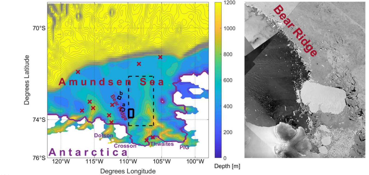
Figure 1: Left: Amundsen Sea and Bear Ridge topography [m] based on the BedMachine Antarctica dataset (Morlighem et al., 2020) and re-gridded on the model configuration grid. Gray contours are spaced 80 m apart. Thin solid black contours delimit the bounds of boxes a and b in Figure 2, indicating the sites of observed iceberg scours in Section 2.1 with magenta labels matching boxes a and b in Figure 2. Dark red crosses mark the locations of sediment samples analysed in Section 2.2. The thick purple line shows the ice shelf edge, with major ice shelves labelled: Dotson, Crosson, Thwaites, and Pine Island Glacier (PIG). Thick solid (thin dashed) black lines show the boundaries of the boxes where icebergs are released in the SHORT (LONG) simulations. Right: Copernicus Sentinel-1 SAR (synthetic aperture radar) image from 12 February 2022 over Bear Ridge with white shades indicating the presence of icebergs and sea-ice.
