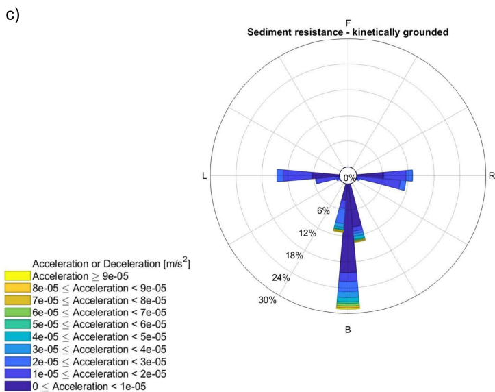
Figure 13: As Figure 12 but for the gravitational acceleration and the deceleration due to dissipative forces in the case of kinetic grounding of THICK icebergs: (a) gravitational acceleration present in a small fraction of the iceberg timestep samples (b), the Coulomb solid-body frictional deceleration (c), deceleration due to kinetic sediment resistance. Occasionally, the orientation of the deceleration due to sediment resistance force is not strictly against the iceberg motion for numerical reasons: the force is calculated using the projected directions of future motion at each Runge-Kutta stage of the iceberg dynamics algorithm.
