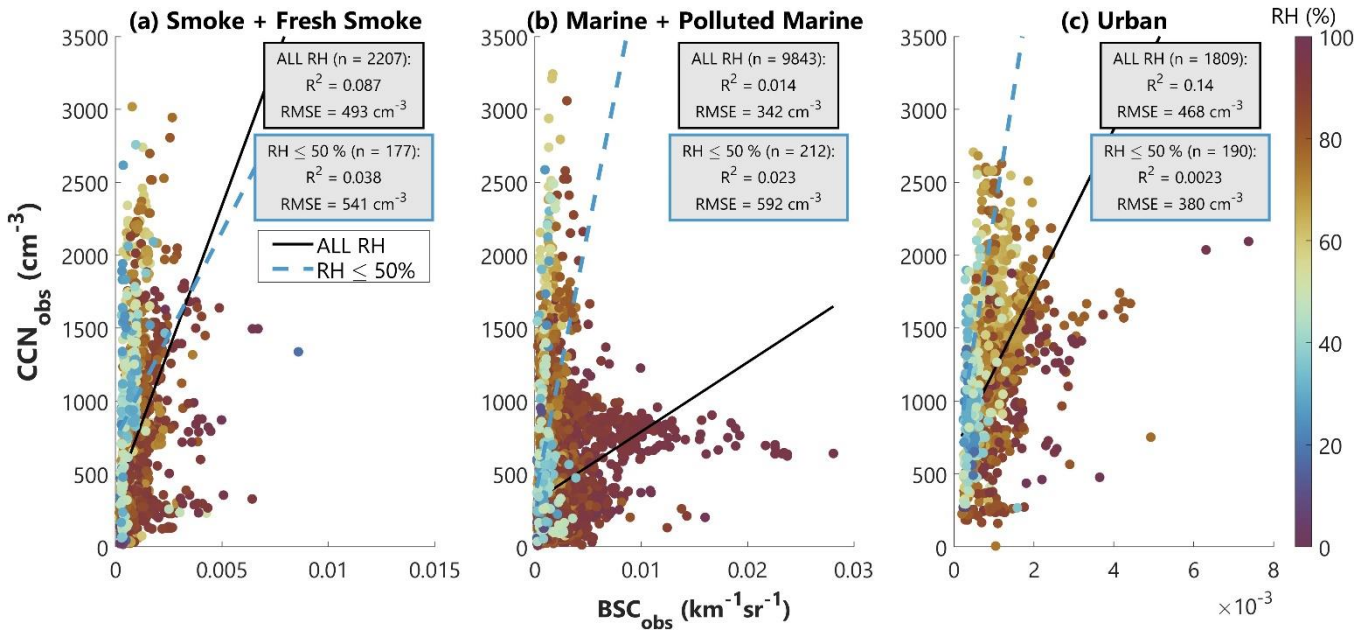
150 Figure 2: Bisector regression of CCN_{obs} vs. BSC_{obs} at 532 nm for (a) smoke and fresh smoke, (b) marine and polluted marine, and (c) urban aerosols. This combined data set covers all years of ACTIVATE and represents 76 flight days. Supersaturation for these observations ranges between 0.36-0.38%. The number of collocated data points (n) is given, as well as the R^2 value and root mean square error (RMSE). Statistics are given for the full data set (black-outlined box), as well as the subset of data observed at RH \leq 50\% (blue-outlined box). The solid black line of best fit applies to 155 the full data set, and the dashed blue line of best fit applies to the low RH subset of data.
