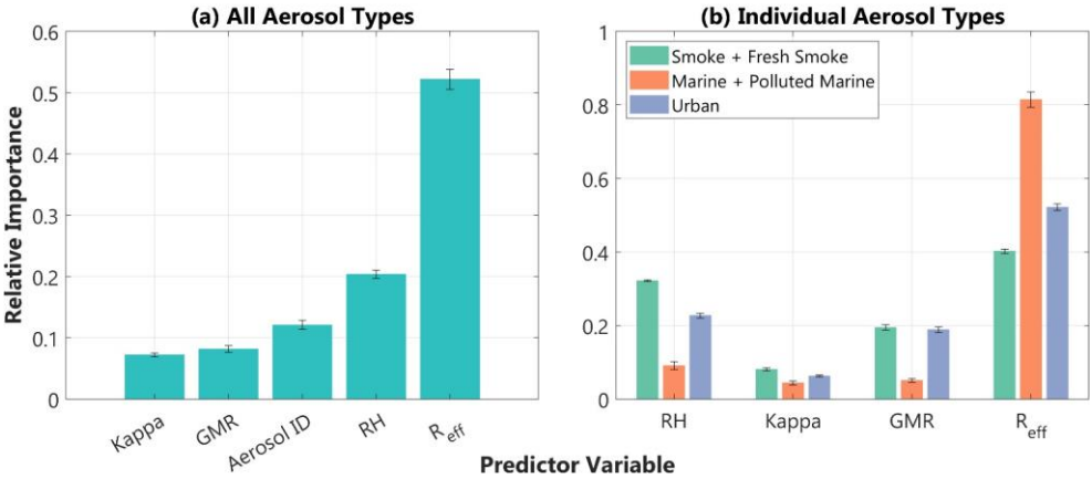
Figure 7: Average random forest predictor importance estimates across 10-fold cross-validation for (a) the model run for a combination of aerosol types combined and (b) individual models run for the three different aerosol types. Each
