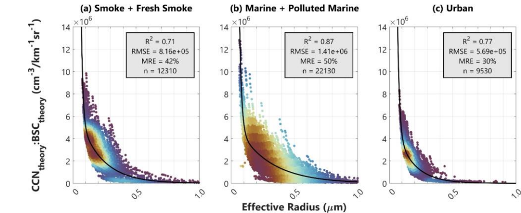
Figure 8: CCN_{theory}:BSC_{theory} vs. R_{eff} for (a) smoke and fresh smoke, (b) marine and polluted marine, and (c) urban aerosols. Marker colors correspond to the density of surrounding points, with red shades indicating high density and blue shades indicating lower density. The black line represents the two-term exponential curve fit for each aerosol type. R^2 , RMSE, mean relative error (MRE) , and number of data points (n) for each exponential fit are also provided.
