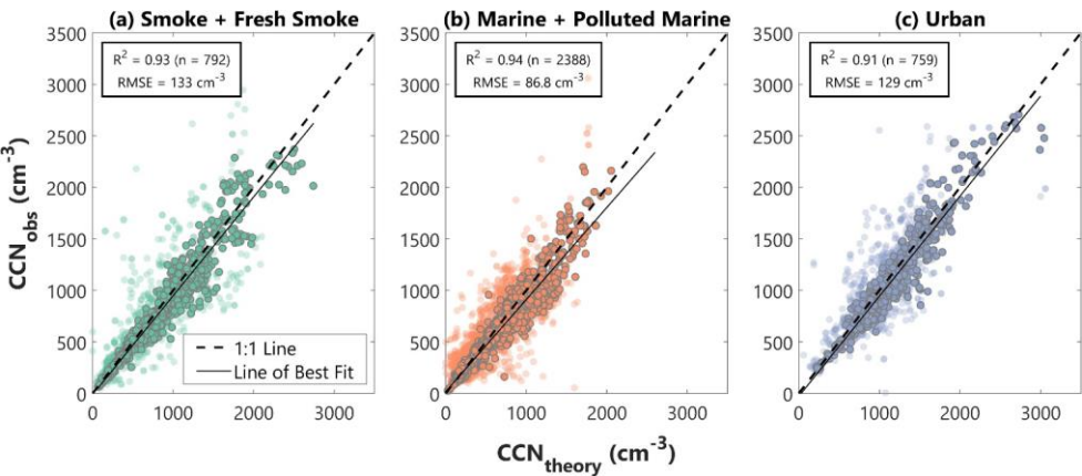
Figure 5: CCN_{obs} vs. CCN_{theory} for (a) smoke and fresh smoke, (b) marine and polluted marine, and (c) urban aerosols. The 1:1 lines are dashed, and the lines of best fit for the linear regressions between both variables are solid. Markers outlined in gray denote results for calculations requiring a certain level of D_{crit} agreement. Results for calculations not requiring a D_{crit} agreement are shown in the background with lighter transparency to demonstrate how this requirement impacts the data set.
