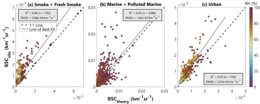
Figure 6: BSC_{obs} vs. BSC_{theory} at 532 nm for (a) smoke and fresh smoke, (b) marine and polluted marine, and (c) urban aerosols. The 1:1 lines are dashed, and the lines of best fit for the linear regressions between both variables are solid. Marker colors correspond to ambient RH that was observed by each BSC_{obs} and applied to calculate each corresponding BSC_{theory} .
