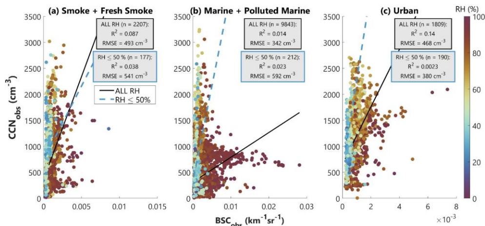
Figure 2: Bisector regression of CCN_{obs} vs. BSC_{obs} at 532 nm for (a) smoke and fresh smoke, (b) marine and polluted marine, and (c) urban aerosols. This combined data set covers all years of ACTIVATE and represents 76 flight days. Supersaturation for these observations ranges between 0.36–0.38%. The number of collocated data points (n) is given, as well as the R^2 value and root mean square error (RMSE). Statistics are given for the full data set (black-outlined box), as well as the subset of data observed at RH \leq 50\% (blue-outlined box). The solid black line of best fit applies to the full data set, and the dashed blue line of best fit applies to the low RH subset of data.
