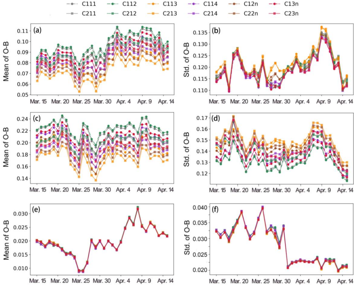
260 Figure 3. Time series of the O-B biases and standard deviations for (a-b) all, (c-d) cloudy, and (e-f) clear pixels. The results are for the CM-FY-DM experiment.
