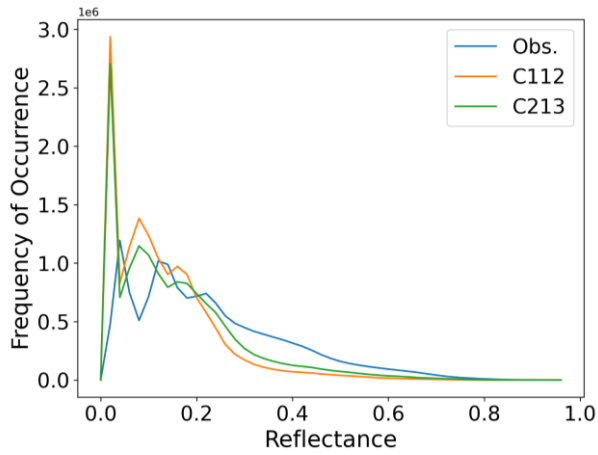
270 Figure 4. The Probability density Distribution Functions (PDFs) of reflectance for the observed and synthetic images from March 15 to April 15 in 2024.
