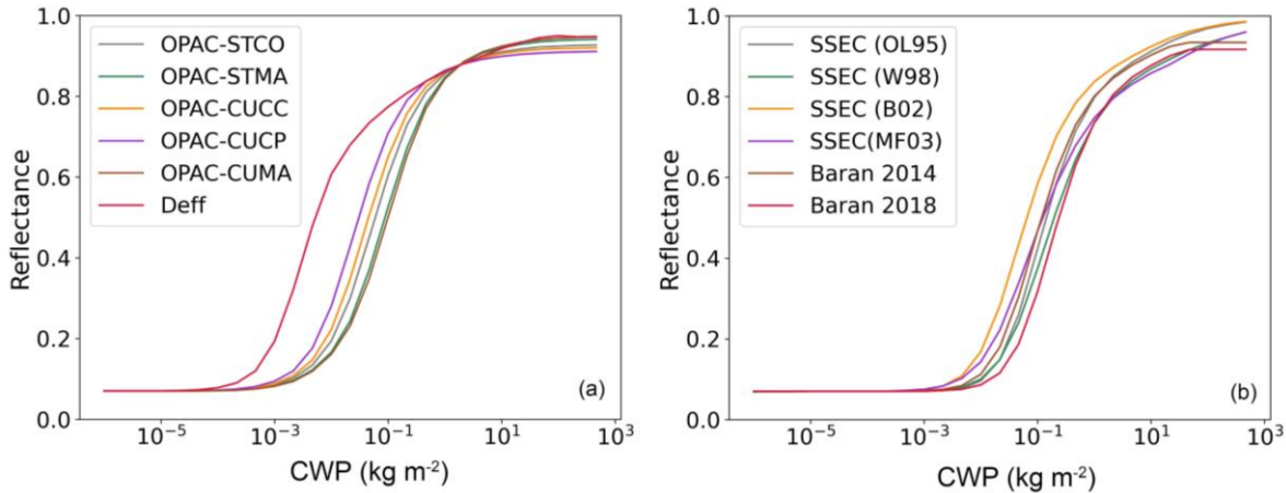
280 Figure 5. Dependence of FY-4B/AGRI band 2 reflectance on cloud water path (CWP) for different (a) liquid water cloud optical parameterizations and (b) ice cloud optical parameterizations. For this simulation, the solar zenith angle, viewing zenith angle, and relative azimuth angle are set to 25 °, 40 °, and 135 °, respectively.
