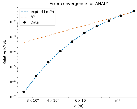
Figure 4. Relative error against resolution measured by effective grid size h from the ANALY experiment. Each black dot represents a simulation with different resolution. The dashed (blue) curve represents a best fit curve to an exponential. The dotted (orange) curve is a third-degree monomial representing third-order error convergence as an upper bound for the theoretical error. The actual error drops exponentially faster with increasing resolution that is decreasing grid size.
