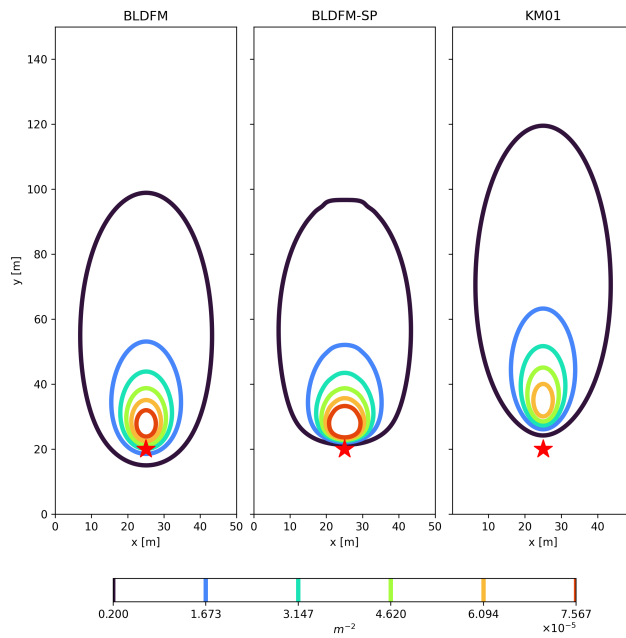
Figure 6. Footprints of BLDFM and the Kormann and Meixner footprint model under very unstable conditions of the atmospheric boundary layer (see Section 7.3 for more details).
