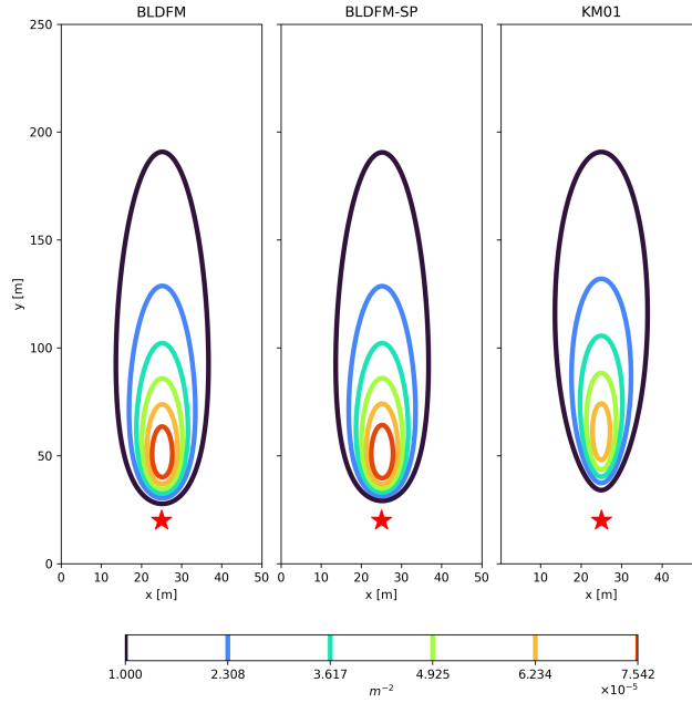
Figure 4. Footprints of BLD FM, modified BLD FM-SP with slender plume approximation and the Kormann and Meixner footprint model (KM01), subject to neutral stability conditions of the atmospheric boundary layer. The red stars mark the position of the receptor (see Section 7.1 for more details).
