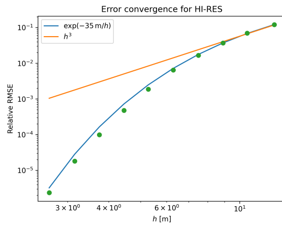
Figure 3. Relative error against effective grid size h from the HI-RES experiment. Each green dot represents a simulation with different resolution. The blue line represents a best fit curve to an exponential. The orange line is a third degree monomial.
