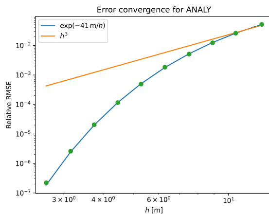
Figure 2. Relative error against effective grid size h from the ANALY experiment. Each green dot represents a simulation with different resolution. The blue line represents a best fit curve to an exponential. The orange line is a third degree monomial.
