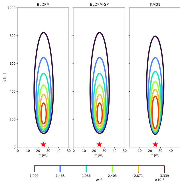
Figure 5. Footprints of BLDFM and the Kormann and Meixner footprint model under very stable conditions of the atmospheric boundary layer (see Section 7.2 for more details).
