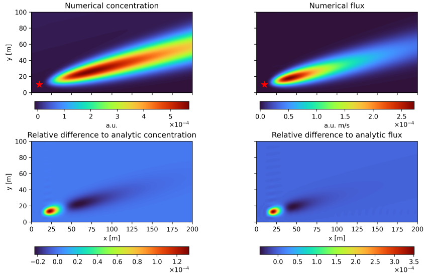
Figure 1. Comparison with analytical solution for constant profiles of horizontal wind and eddy diffusivities. Top row: concentration and flux at 10 m computed with the BLDFM numerical scheme arising from a surface unit point source at the red star. Bottom row: relative differences to the analytic solution.
