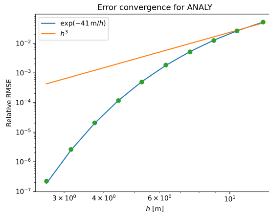
Figure 2. Footprints of BLDFM and Relative error against effective grid size h from the Kormann and Meixner footprint model, subject ANALY experiment. Each green dot represents a simulation with different resolution. The blue line represents a best fit curve to very-unstable conditions of the atmospheric boundary layer (see text for more details) an exponential. The orange line is a third degree monomial.
