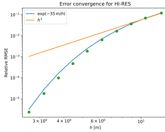
Figure 3. Footprints of BLDFM and Relative error against effective grid size h from the Kormann and Meixner footprint model under very stable conditions of the atmospheric boundary layer (see text for more details) HI-RES experiment. Each green dot represents a simulation with different resolution. The blue line represents a best fit curve to an exponential. The orange line is a third degree monomial.
