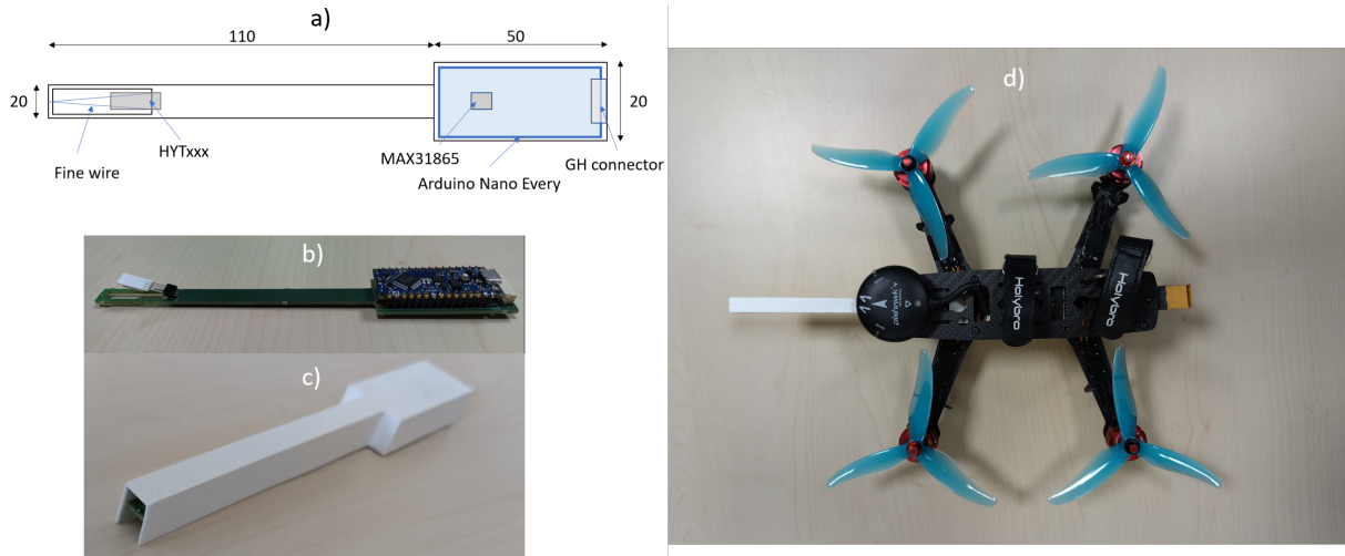
Figure 1. SWUF-T board design concept (a) and pictures of the sensor without (b) and with (c) housing. (d) shows the sensor attached to the QAV250 UAS frame.
