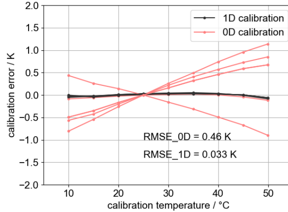
Figure 4. Calibration error of 5 FWPRT sensors with respect to the reference sensor in the calibration chamber after 0 D calibration (bias correction at 25°C, red curves) and 1 D calibration (grey curves).
