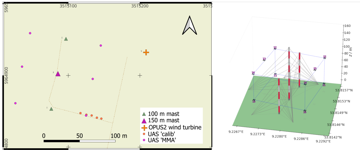
Figure 2. Left: Map of the Krummendeich test site with wind turbine OPUS2 (orange cross), MMA (triangles) and drone flight positions (purple and orange circles). Background map: ©OpenStreetMap contributors 2025. Distributed under the Open Data Commons Open Database License (ODbL) v1.0. Right: The MMA-pattern in a 3D representation.
