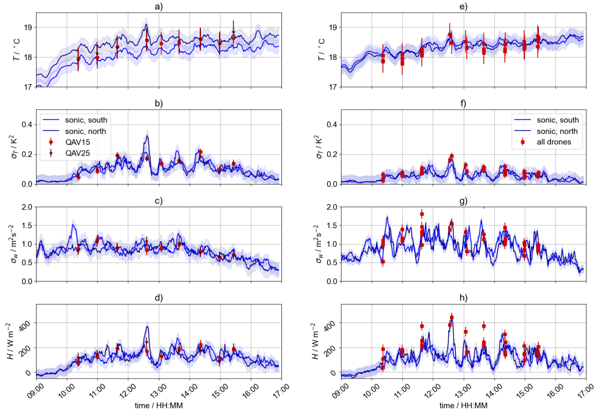
Figure 12. Time series of temperature T (a,e), temperature variance \sigma_T^2 (b,f), vertical wind speed variance \sigma_w^2 (c,g) and sensible -heat flux H (d,h) for 22 July 2024. 10-minute averaged sonic anemometer measurements on south (dark blue) and north mast (light blue) are compared to drone measurements (red squares).
