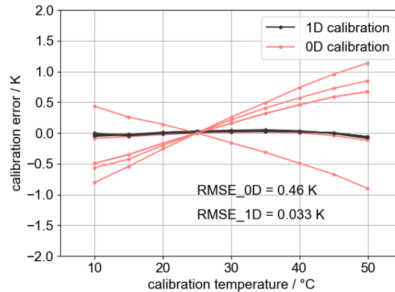
Figure 5. Calibration error of 5 FWPRT sensors with respect to the reference sensor in the calibration chamber after 0 D calibration (bias correction at 25°C, red curves) and 1 D calibration (grey curves).
