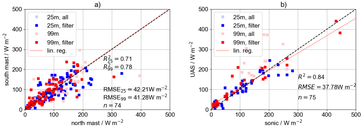
Figure 11. Comparison of sensible heat flux between sonic anemometers of north and south mast (a) and between UAS and the closest mast (b). Shown are the comparisons at 25 m level (blue) and 99 m level (red). The linear regression is shown as red dotted line.
