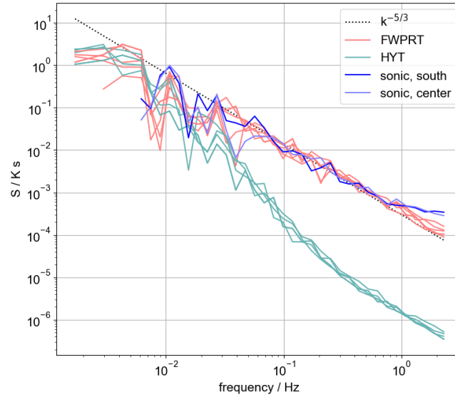
Figure 9. Spectra of virtual-sonic temperature for one-UAS flight #70 next to a sonic anemometer showing measurements of the sonic ( grayblue ), the slow HYT271 ( bluegreen ) sensor and the FWPRT (red).
