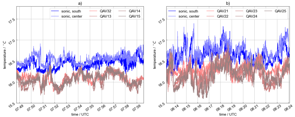
Figure 7. Time series of virtual temperature for four five UAS (red) in close proximity to the met mast array and corresponding sonic anemometer readings (blue) for flight #70-69 (a) and #70 (b). Comparison of mean virtual temperature measurements with UAS compared to corrected sonic temperature on closest mast.
