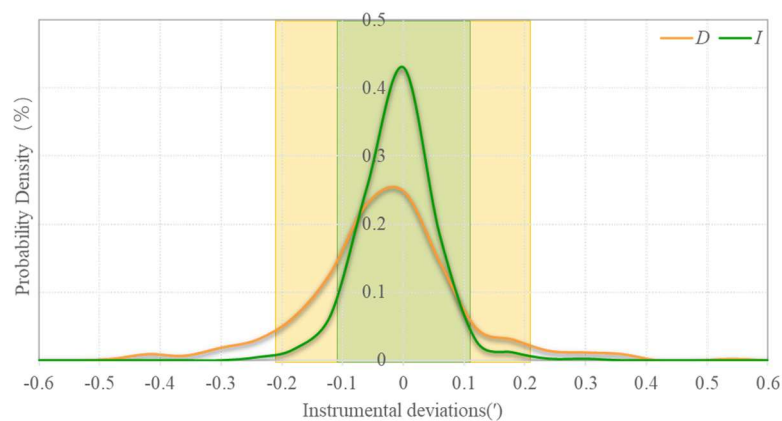
Figure 3: The instrument differences of declination D (orange line) and inclination I (green line).
