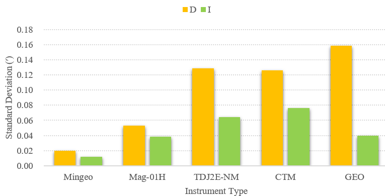
Figure 5: The standard deviation of the instrument differences for five types of instruments.
