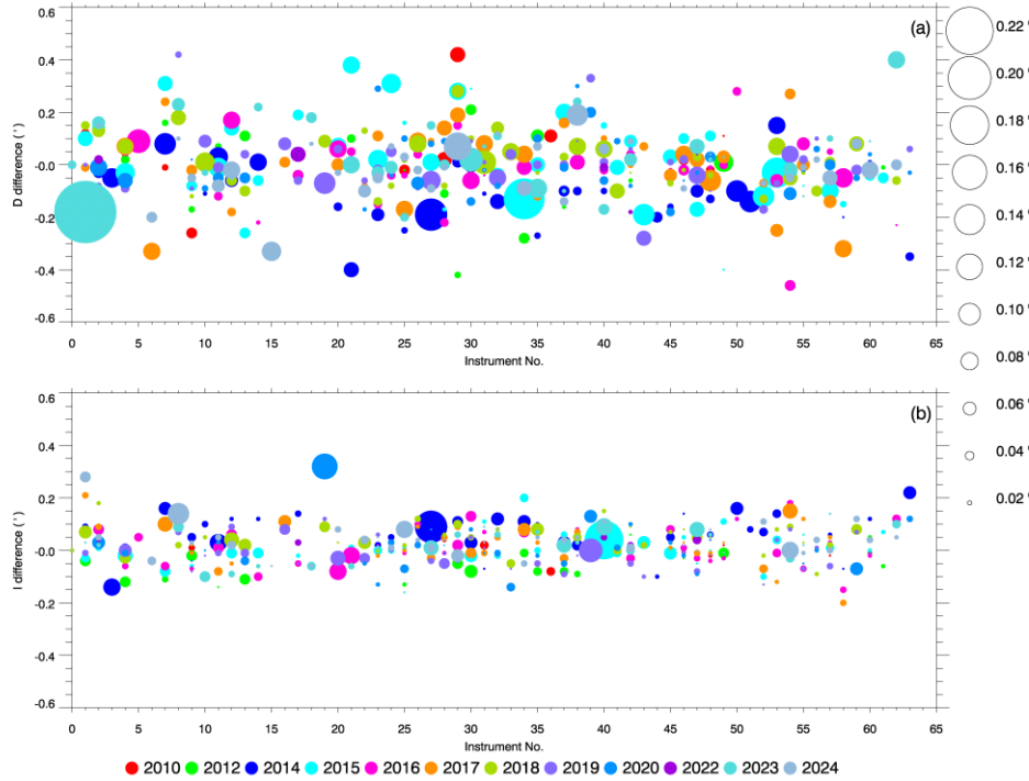
Figure 2: Instrumental differences in declination D (a) and inclination I (b). The dots represent the instrument differences; the size of the dots is the standard deviation with the scale on the right. The colors indicate different years.
