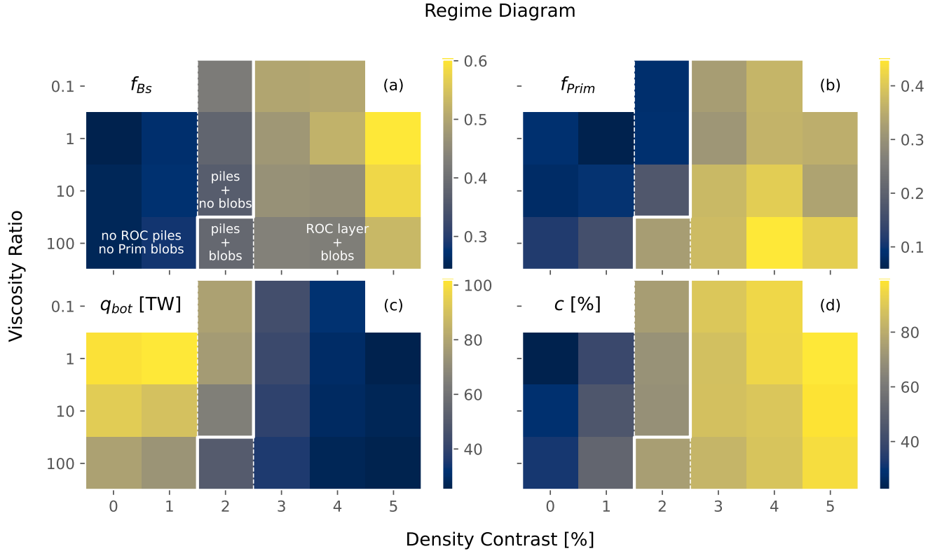
Figure 3. Regime diagram spanning the parameter space of our study (i.e., the viscosity ratio \zeta and the density contrast \Delta\rho_{Bs}/\rho_{Py} between ROC in the LM and the pyrolytic ambient mantle). Panels a, b, c and d Each group of four points represents one case. Different markers represent basalt and primordial fractions, CMB heat-flux and CMB basalt coverage (respectively, f_{Bs} , f_{Prim} , q_{bot} and c ), respectively. All quantities are averaged between 4 Gy and 5 Gy model time. We calculate f_{Prim} and f_{Bs} by averaging across the depth-ranges 720 \text{ km} \leq z \leq 2400 and 2400 \text{ km} \leq z \leq 2890 \text{ km} , respectively. We calculate c as the fraction of cells above the CMB with f_{Bs} > 0.5 . Heavy and thin lines represent the boundaries between regimes and sub-regimes, respectively. The boundary between the main regimes 'Mixed Prim' and 'Prim Blobs' (i.e., M and B respectively) is drawn by setting the threshold f_{Prim} = 0.3 and is indicated with a full line. The sub-regimes are characterized as having 'No Piles', 'deep ROC Piles' and a 'deep ROC Layer'. Boundaries between these sub-regimes are drawn by setting c = 0.6 and c = 0.8 , and are indicated with a dashed line (for M0 to MP/BP and for MP/BP to BL, respectively). Regime labels appear only in panel a to avoid clutter.
