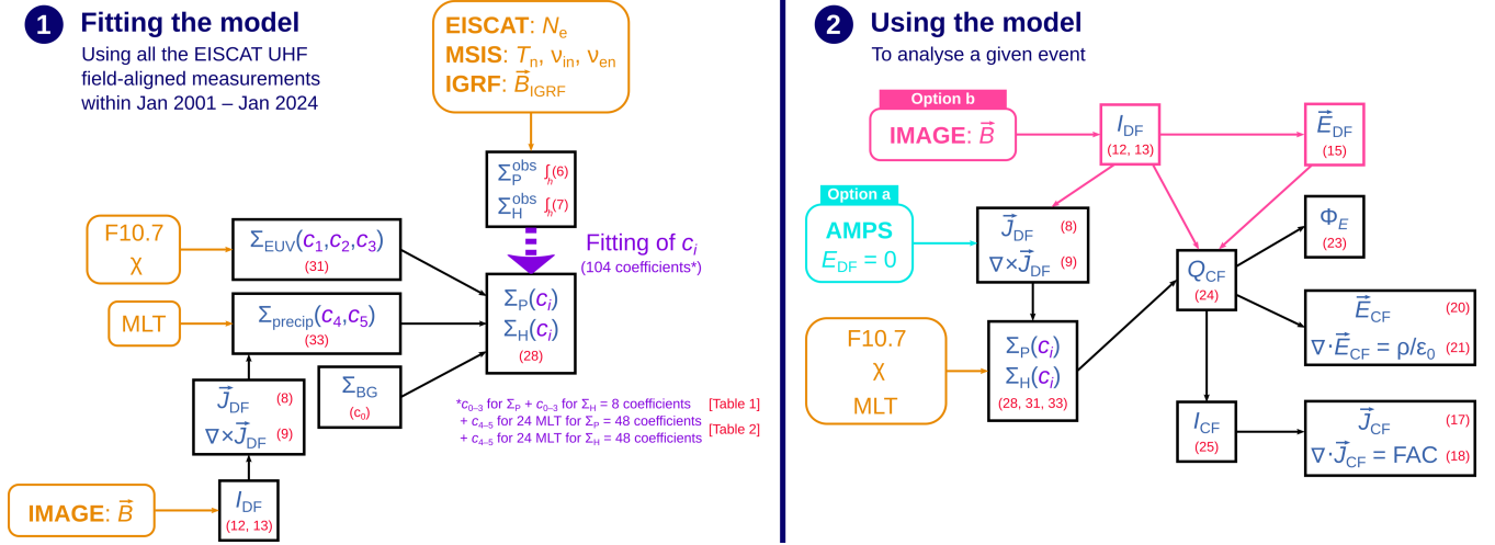
Figure 7. Summary of fitting of the Ebec model (1) and of using the Ebec model (2). Input data are in yellow, derived parameters in blue, model coefficients in purple, and equation numbers in red. The right hand side illustrates how the model is used in section 3.2 (“Option a”, cyan color) and section 3.3 (“Option b”, pink color).
