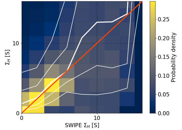
Figure 8. The same as Fig. 6a–d except that instead of the new EISCAT-based model Ebec , values modelled using SWIPE are compared with the EISCAT observations.
