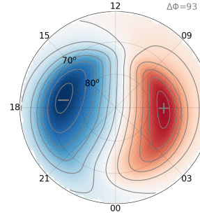
(e) SWIPE electric potential
