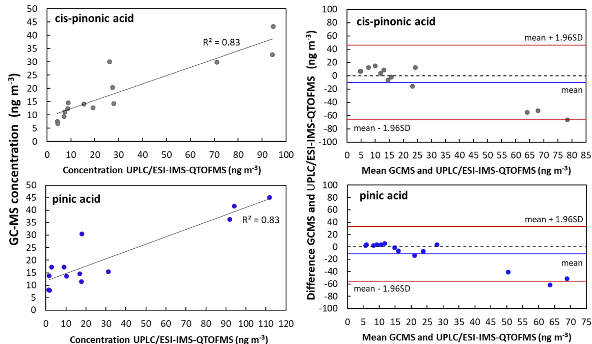
Figure 6. Concentration plots for cis-pinonic acid and pinic acid and Bland-Altman plots for comparison of UPLC/ESI-IMS-QTOFMS and GC-MS methods. Analysis was performed on aerosol samples collected at the Rambouillet forest (France) during the summer 2022. Bland-Altman plots show the difference between UPLC/ESI-IMS-QTOFMS and GC-MS methods. Black and blue lines show the mean of the difference between measurements and red lines represent the upper and lower limits of agreement, which were calculated considering 1.96 times the standard deviation (Bland and Altman, 1999).
