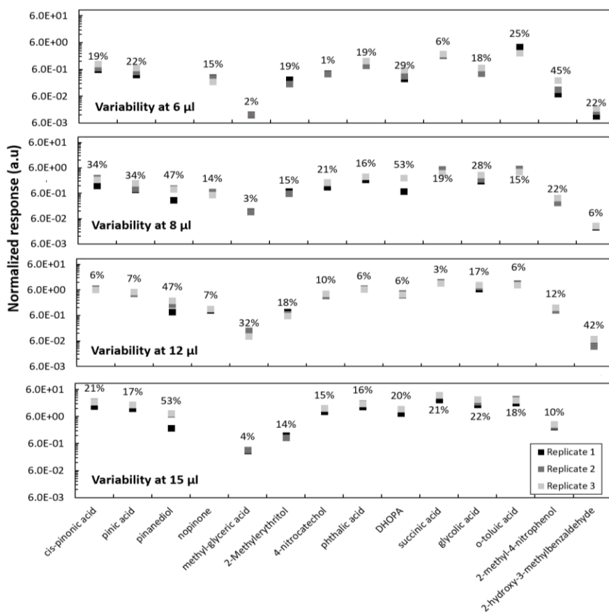
Figure 4. Replicates variability at different injection volumes of 6, 8, 12 and 15 µl from a mixture solution of anthropogenic and biogenic standards at 50 \mu\text{g mL}^{-1} analyzed in the GC-MS. Transition time between replicates injection varies between 3 and 4 days. Compound responses are normalized to the internal standard response.
