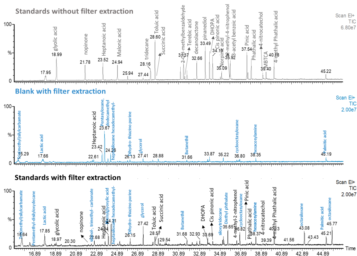
Figure 3. TIC Chromatogram of a mixture of anthropogenic and biogenic compounds injected directly in the GC-MS after derivatization without filter extraction (top panel) and with filter extraction (bottom panel). The middle panel accounts for the blank filter extraction. In the bottom panel, peak assignment for the standards compounds is highlighted in black color, while blue represent the peak identification performed with the NIST library.
