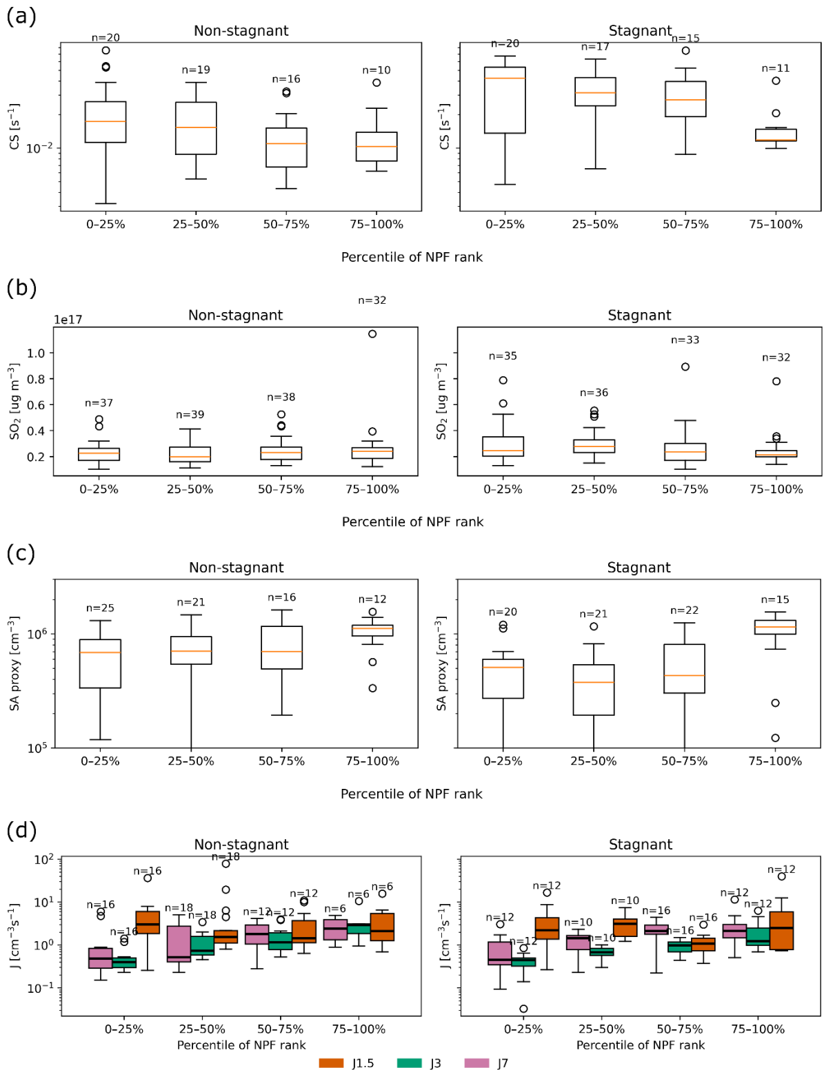
Figure S9: Daily a) median CS, b) median SO_2 , c) median SA proxy calculated over the active time window of each day per rank class during stagnant and non-stagnant conditions; d) daily maximum J_{1.5} , J_3 , and J_7 during the active window of each day, per rank class during stagnant and non-stagnant conditions. n indicates the number of datapoints included in the boxplot. For the description of the boxplot, see Fig. 4b.
