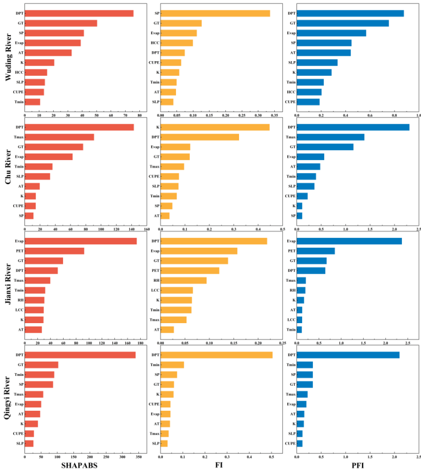
Fig. 14 Bar plots showing the importance ranking of hydrometeorological variables across the four river basins based on the TCN-GRU model (evaluation metrics: SHAPABS, FI, PFI). Additionally, interpretability analysis for extreme events revealed significant stage differences:
