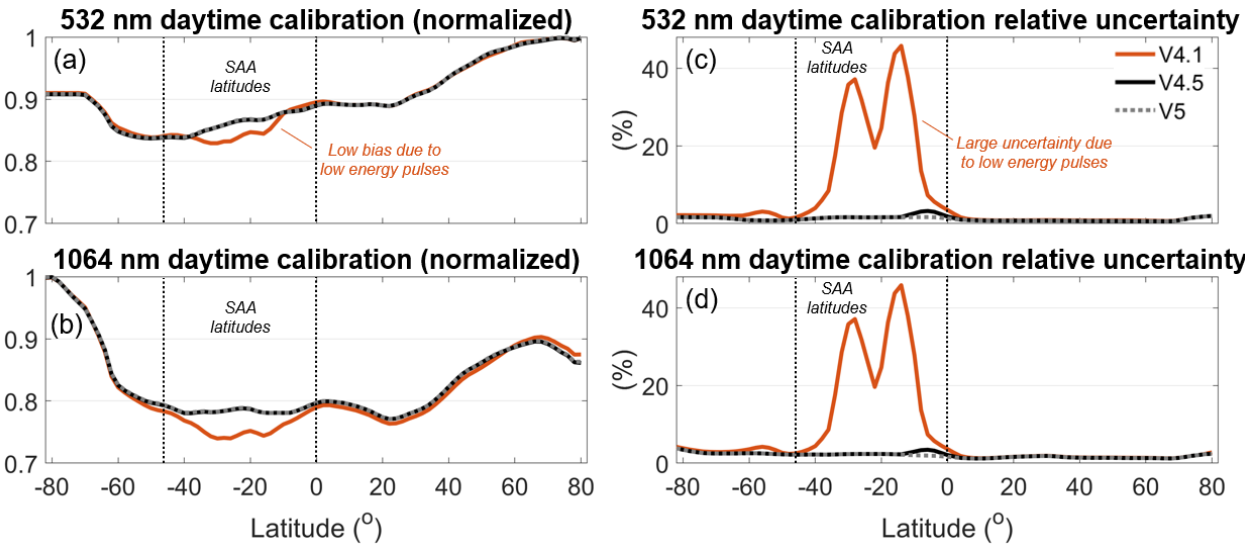
Figure 8. Zonal mean daytime (a, b) calibration coefficients and (c, d) calibration relative uncertainties for the 532 nm and 1064 nm channels in the V4.1, V4.5, and V5 data releases for November 2020. Calibration coefficients are normalized by the maximum of all three versions.
