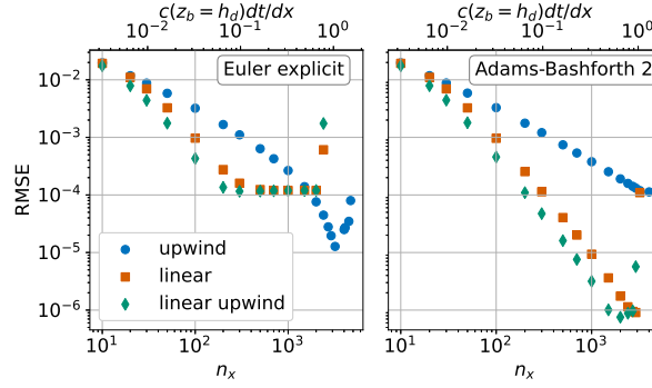
Figure 12. Root mean square error for different combinations of numerical schemes and mesh refinements. The time step is constant ( \delta t = 0.05\text{s} ) for all simulations, with only the number of faces ( n_x ) in the finite area mesh varying. The maximum Courant number, based on the bedform celerity, is indicated on the top axis.
