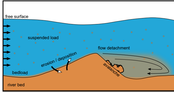
Figure 1. Schematic representation of the flow above a riverbed and the main sediment transport processes involved.
