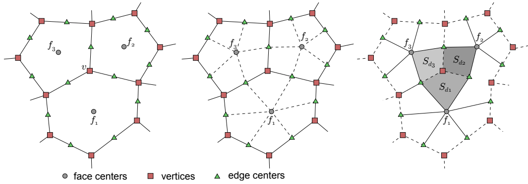
Figure 3. Construction of the dual mesh from the horizontal projection of the finite-area mesh. The dual mesh is formed by connecting the centers of the original mesh faces and the centers of their edges, illustrated here for three polygonal faces.
