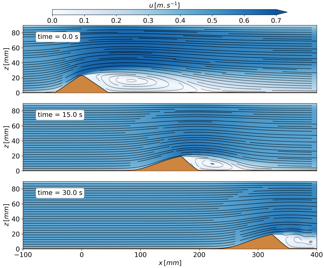
Figure 18. Representation of the dune at different times (0, 15, and 30 seconds) during the migration process. The flow streamlines highlight flow detachment near the dune crest and the recirculation cell downstream. Starting from an initial conical shape, the dune evolves into an asymmetric stationary form.
