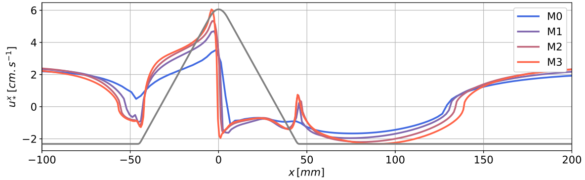
Figure B1. Comparison of streamwise component of friction velocity obtained for 4 different mesh resolutions (M0, M1, M2, and M3).
