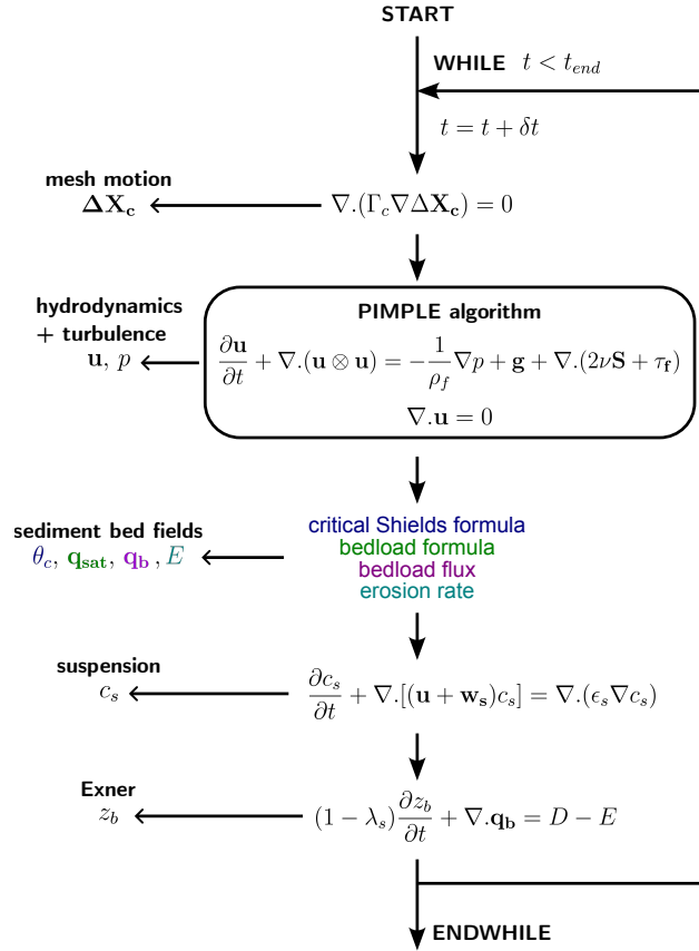
Figure 2. Flow chart of sedExnerFoam , illustrating the operations performed by the model during each time iteration.
