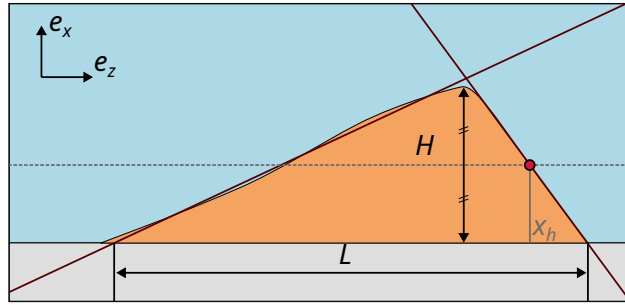
Figure A1. Schematic showing how the dune’s characteristics are defined. The dune’s position is tracked using the coordinate x_h corresponding to the abscissa of the mid-height of the downstream side of the dune. The dune’s length is the base of the triangle formed by the lines approximating the downstream and upstream slopes and the rigid bed.
