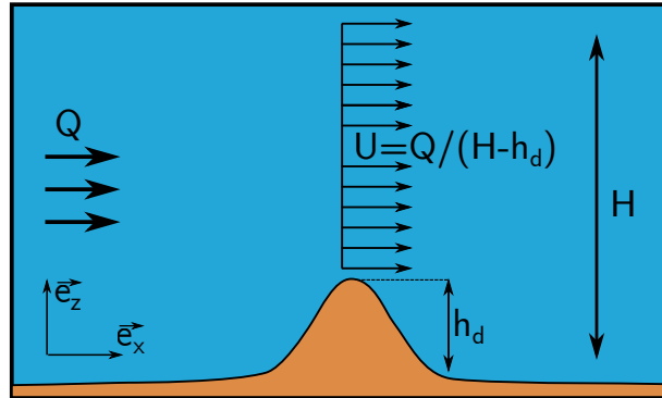
Figure 9. Schematic of the idealized dune migration case showing the main parameters and illustrating the relationship between bed elevation and depth-averaged velocity.
