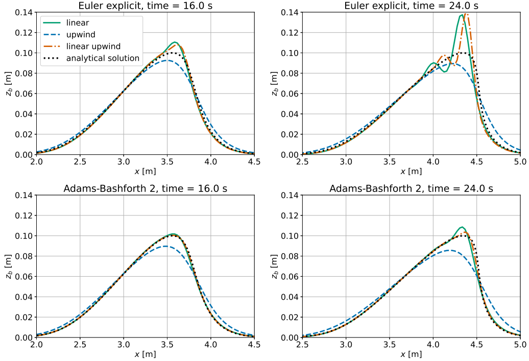
Figure 11. Comparison of bed levels in an idealized dune migration obtained from numerical simulations using three different advective schemes and two temporal integration schemes ( Euler explicit top, Adams-Bashforth 2 bottom) with the analytical solution at intermediate (left) and near-breaking (right) times.
