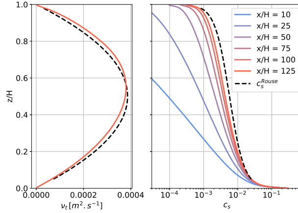
Figure 8. On the left-hand side, the turbulent eddy viscosity obtained with the model (solid line) and the theoretical parabolic profile (black dashed line). On the right-hand side, vertical profiles of c_s at different x -positions in the channel. For comparison, the Rouse profile corresponding to the pseudo-analytical solution in Figure 7 is also plotted (black dashed line).
