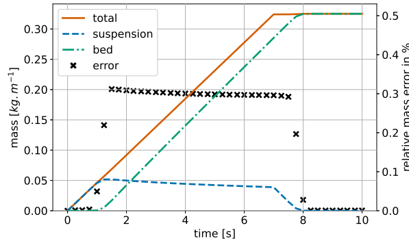
Figure 15. Temporal evolution of sediment mass per unit area, divided into suspended and deposited components, for sand settling in an hourglass. Relative error in total mass (%) is shown by black crosses. Suspended sediment is injected during the first 7 s and fully deposited before the end of the simulation.
