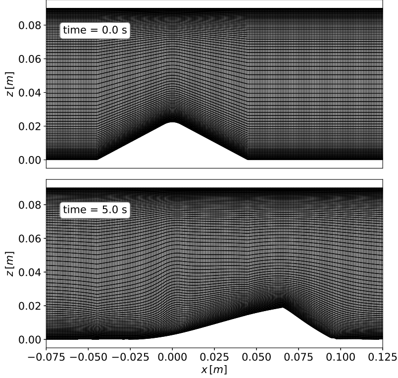
Figure 17. Representation of the dune mesh at different times during the migration process.
