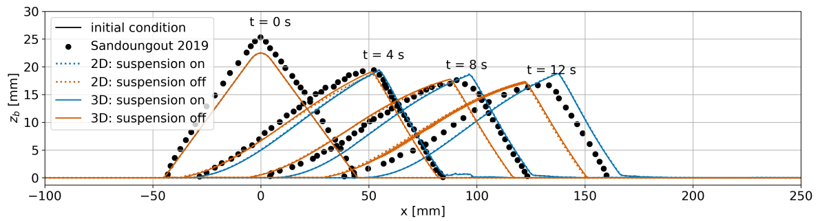
Figure 23. Sediment bed elevation at different times, 0, 4, 8, and 12 seconds. Comparison between the results from 2D and 3D simulations with and without suspension and experimental results.
