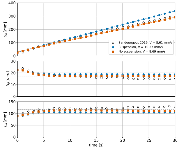
Figure 20. Dune morphological parameters evolution in time. From top to bottom are plotted the dune position represented by the coordinates x_h , which is located halfway up the downstream face of the dune, as well as the dune height h_d and the dune length L_d . In the top panel, the dashed lines represent the linear fit of the numerical results from which the dune migration speed is estimated as the slope of the linear regression.
