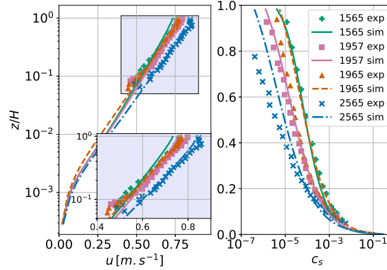
Figure 5. Velocity and suspended sediment concentration profiles from numerical simulations and comparison with experimental data from Lyn (1988).
