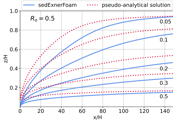
Figure 7. Isolines of c_s/c_b^* . Comparison between pseudo-analytical solution from Hjelmfelt and Lenau (1970) (red dotted lines) and the model solution (solid blue lines) without enforcement of the assumptions used to derive the pseudo-analytical solution.
