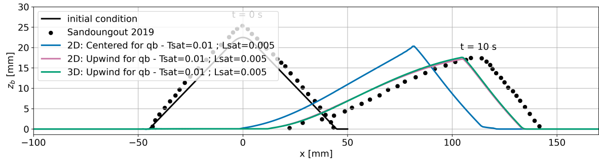
Figure C1. Bed elevation obtained with different advection schemes for the divergence of bedload flux in the Exner equation: Upwind and Linear (Centered) schemes, coupled with a second order Adams-Bashforth scheme for the time derivative. The saturation length value is fixed to L_{sat} = 5 \text{ mm} and the saturation time is fixed to T_{sat} = 0.01 \text{ s} .
