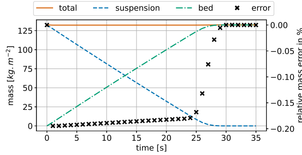
Figure 13. Time evolution of sediment mass per unit area, divided into suspended and deposited fractions, during deposition in a still basin. Relative error (%) of the total mass is shown by black crosses.
