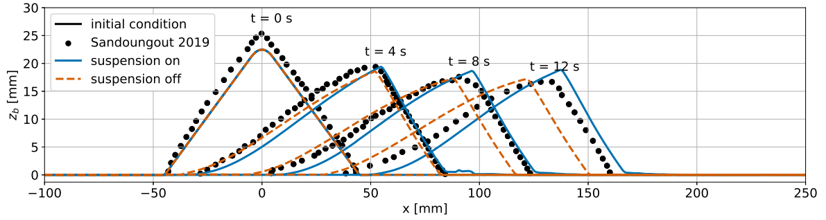
Figure 19. Sediment bed elevation at different times, 0, 4, 8, and 12 seconds. Comparison between the results from two simulations and experimental results. The simulations use the same mesh, same parameters, but for one, the suspended load is not taken into account.
