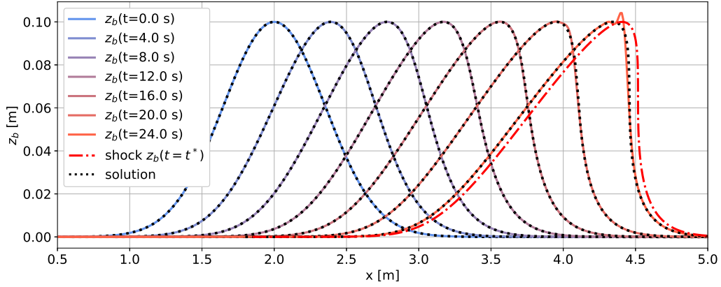
Figure 10. Bed level evolution of an initially Gaussian dune during an idealized transport scenario, comparing model results (solid lines) with the analytical solution (black dotted lines).
