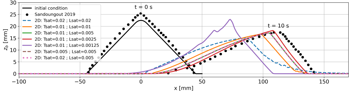
Figure 21. Bed elevation obtained with different saturation length values, ranging from L_{sat} = 1.25 \text{ mm} to L_{sat} = 20 \text{ mm} with saturation time T_{sat} = 0.01 \text{ s} except for L_{sat} = 20 \text{ mm} where T_{sat} = 0.02 \text{ s} (due to numerical stability condition) and 2 configurations with T_{sat} = 0.005 \text{ s} and T_{sat} = 0.02 \text{ s} with L_{sat} = 5 \text{ mm} are also showed. All these configurations have been performed without suspension to limit potential non-linear interactions between bedload and suspended load on the dune migration.
