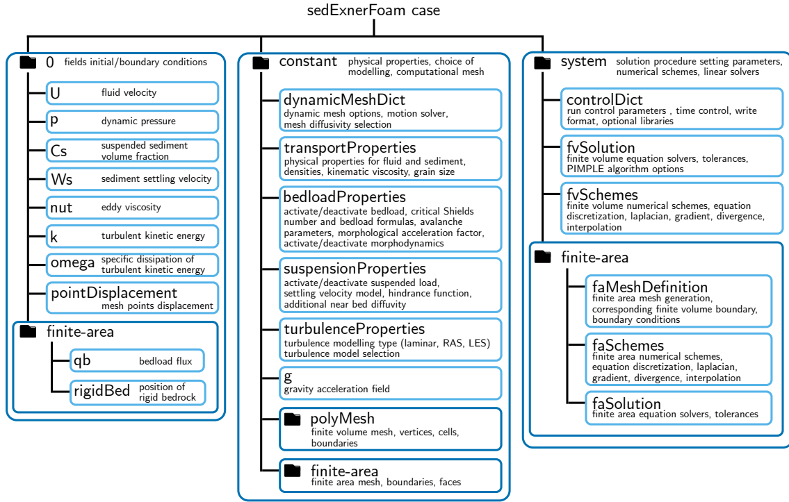
Figure 4. Case directory structure for a sedExnerFoam simulation, organized into three folders: 0 for initial conditions, constant for modeling options and physical properties, and system for time control and numerical settings.
