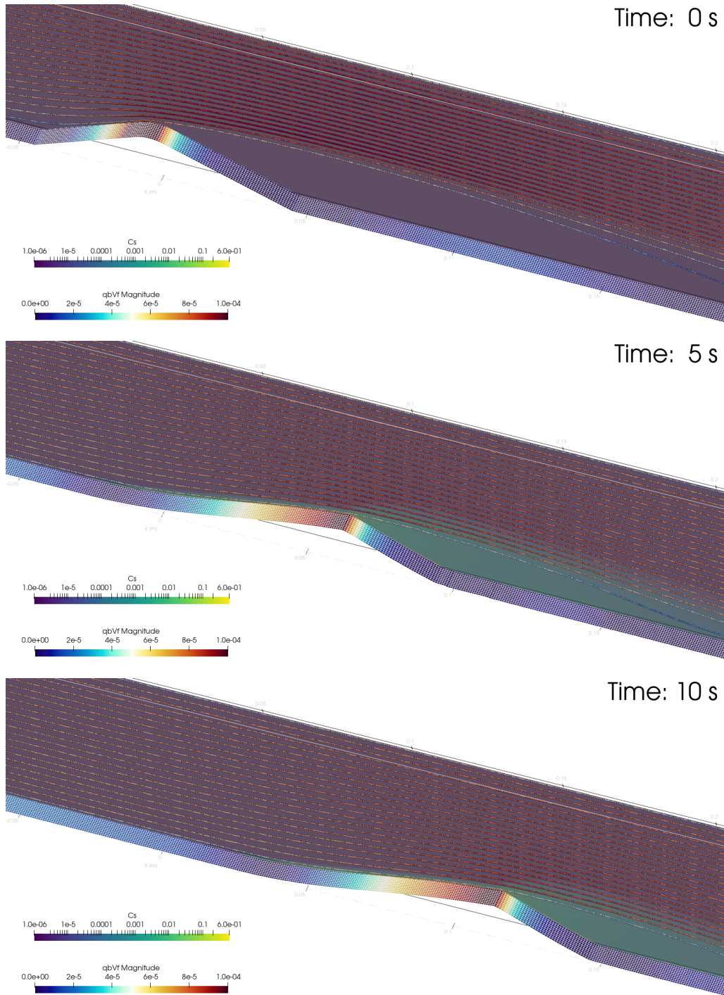
Figure 22. Representation of the dune and the flow streamlines of the 3D configuration at different times, t = 0\text{ s} , 5\text{ s} and 10\text{ s} from top to bottom, during the migration process. The colorplot at the bed represents the saturated bedload flux q_{sat} ( L_{sat} = 0.005\text{ m} and T_{sat} = 0.01\text{ s} ), and the colorplot in a vertical plane represents the suspended concentration c_s in log scale. The streamlines are colored by the flow velocity.
