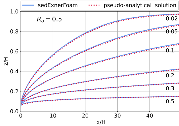
Figure 6. Isolines of c_s/c_b^* for a Rouse number of 0.5 with assumptions from Hjelmfelt and Lenau (1970) enforced except the null horizontal turbulent diffusion. Solid blue curves represent the model results and the dotted red ones the pseudo-analytical solution.
