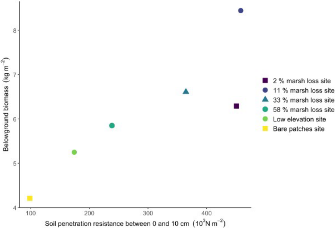
Figure A2: Relation between soil penetration resistance (10³N m⁻²) in the top soil and the belowground biomass (kg m⁻²) for the different field sites.
