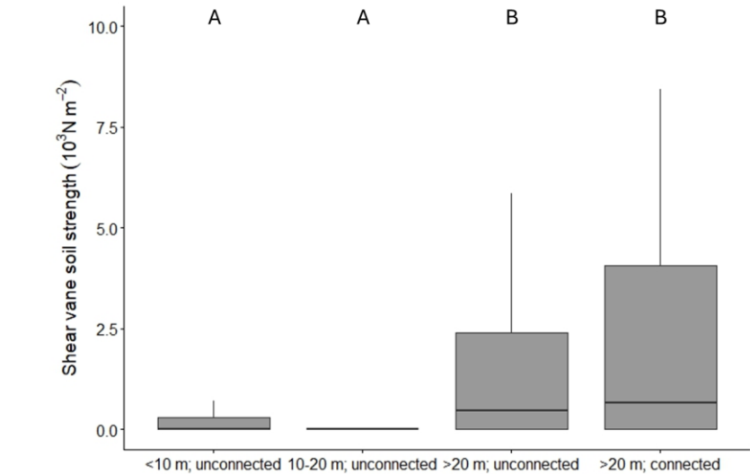
270 Figure 5: Shear vane soil strength ( 10^3 \text{ N m}^{-2} ) measurements of pond topsoils ( n=50 for each boxplot) Significant differences between pond types have different letters above each boxplot, differences between groups have different letters at the very top of the figure (pairwise Wilcoxon rank sum test with Bonferroni correction, \alpha= 0.05 ).
