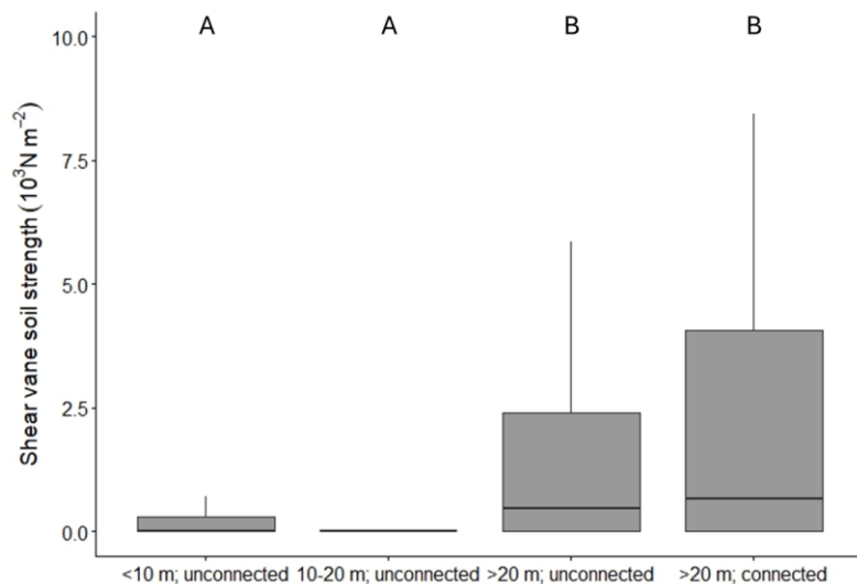
Figure 55: Shear vane soil strength ( 10^3 \text{ N m}^{-2} ) measurements of pond topsoils ( n=50 for each boxplot) and marsh soils at 30 cm depth ( n=25 for each boxplot). Significant differences between pond types or marsh locations have different letters above each boxplot, differences between groups have different letters at the very top of the figure (pairwise Wilcoxon rank sum test with Bonferroni correction, \alpha=0.05 ).
