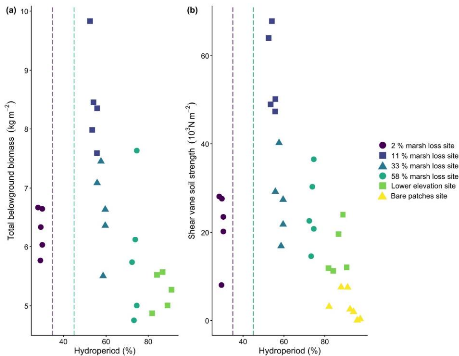
Figure 22: (a) Total belowground biomass ( \text{kg m}^{-2} for 0-15 cm soil depth) versus hydroperiod for all vegetated marsh sampling locations (no bare or pond locations). (b) Top-soil shear vane soil strength ( 10^3 \text{ N m}^{-2} for 0-10 cm soil depth) versus hydroperiod for all vegetated and bare marsh sampling locations (no pond locations). The vertical dashed lines indicate hydroperiods for which belowground biomass production was maximal as determined by an experimental setup close to the 2% and 58% marsh loss sites (Kirwan and Guntenspergen, 2015).
