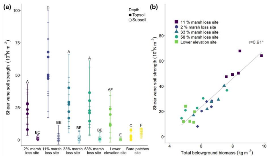
Figure 3: a) Comparison of shear soil strength ( 10^3 \text{ N m}^{-2} , for 0-10 cm soil depth) in the different field locations and between the topsoil (0-10 cm, full circle) and subsoil (30-40 cm, open circle). Letters at the top show the results of the pairwise Wilcoxon rank sum test with Bonferroni correction ( n=25 for each site and depth combination), with different
