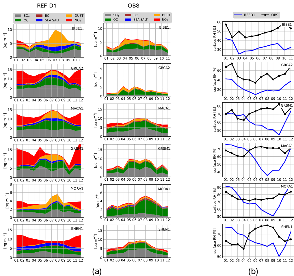
490 Figure 10. Comparison between Ref-D1 and observations for the seasonal cycle of (a) surface PM 2.5 components (a) and (b) surface RH at selected IMPROVE sites. Individual species are measured and compared at RH=0% (dry mass).
