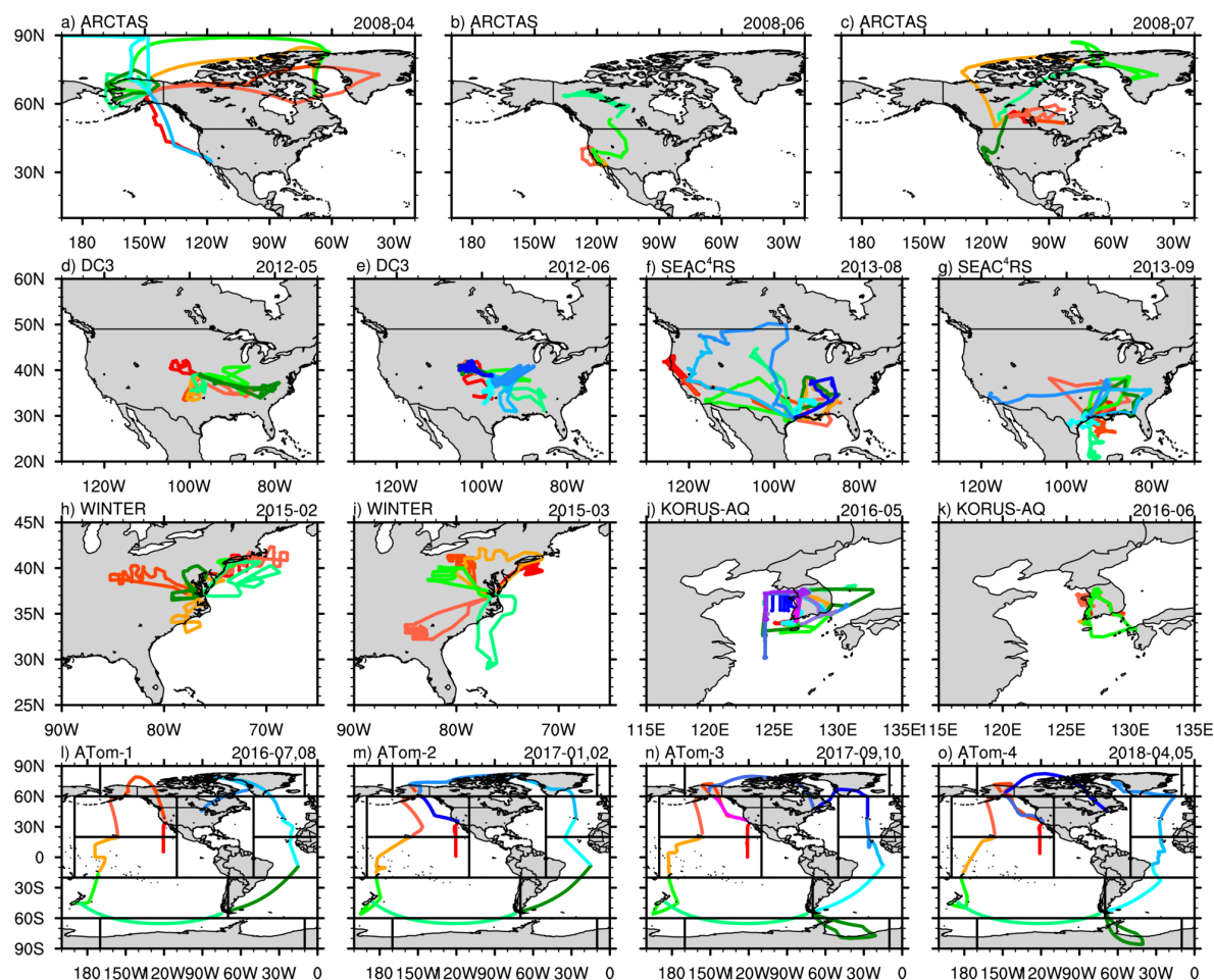
Figure 2: Flight tracks of ARCTAS, DC3, SEAC 4 RS, WINTER, KORUS-AQ, and ATom campaigns. Different colors in each panel 235 represent different flight days during the month(s) noted at the upper-right corner. Black boxes in the bottom-row panels mark the regions used for the average of observations and model results along Atom flight tracks. The latitudes and longitudes of these regions are (60°N-90°N, 170°W-10°W), (20°N-60°N, 170°E-110°W), (20°N-60°N, 50°W-0°), (20°S-20°N, 170°E-110°W), (20°S-20°N, 50°W-0°), (60°S-20°S,
