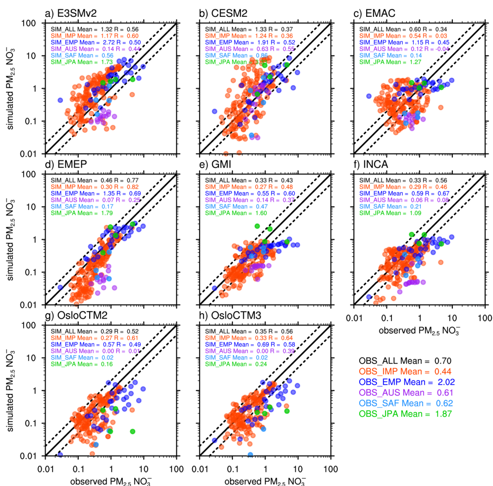
Figure 3: Scatter plots of modeled annual mean PM 2.5 nitrate surface concentrations ( \mu\text{g m}^{-3} ) compared to observations from IMPROVE
