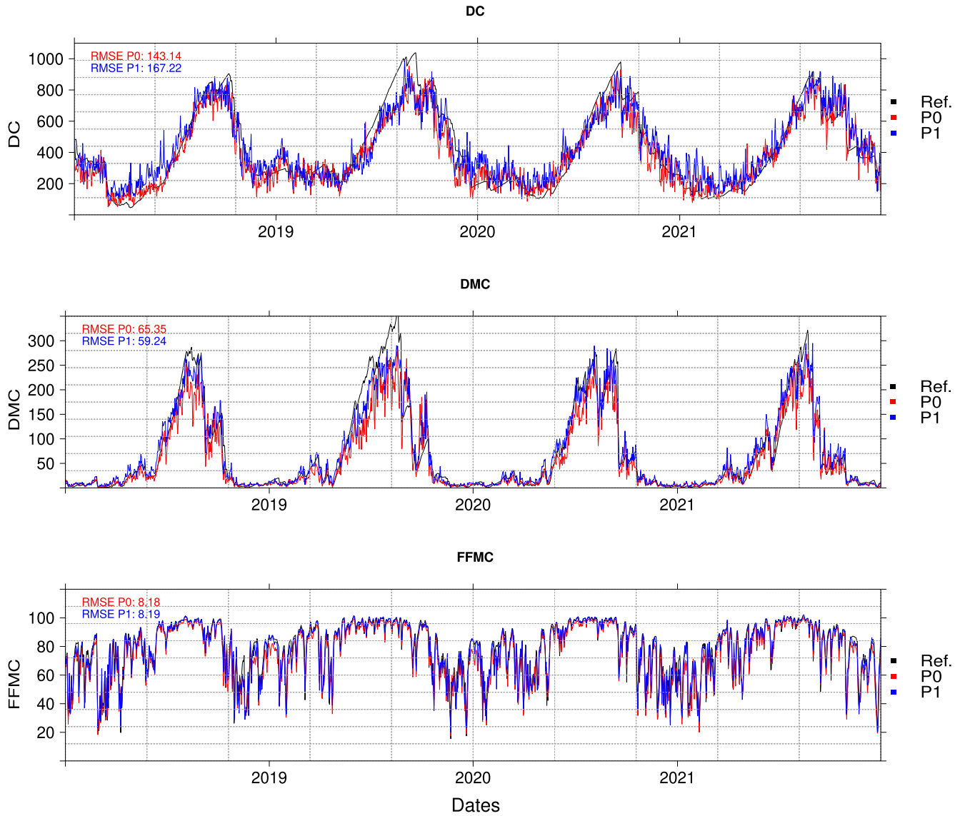
Figure E1. Daily, spatially aggregated time series for the reference, and the DL-based estimates considering the input sets P0 and P1 (see Table 1) over the CONTM region (see Figure A1) during the 2018–2021 test period. The first, second and third row represents the Drought Code, the Duff Moisture Code and the Fine Fuel Moisture Code respectively.
