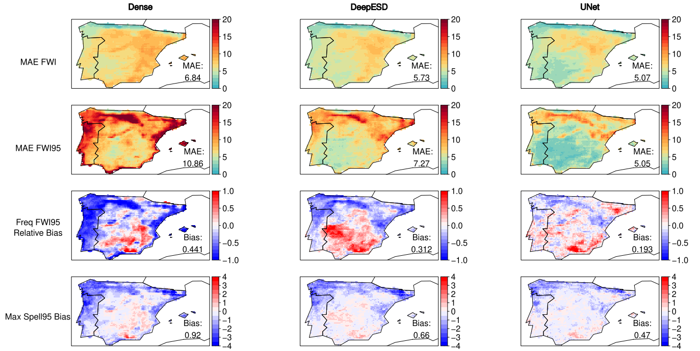
Figure D1. Results from the Dense, DeepESD and U-Net model trained with 12UTC input variables (temperature, 24h-accumulated precipitation, relative humidity and wind speed). The maps display differences relative to the reference FWI for the fire season (June–September) during the test period (2018–2021) for the validation indices. The MAE value inside the map represents the spatially aggregated mean absolute error of the deep learning predictions with respect to the FWI reference, while Bias denotes the spatially averaged bias in absolute value.
